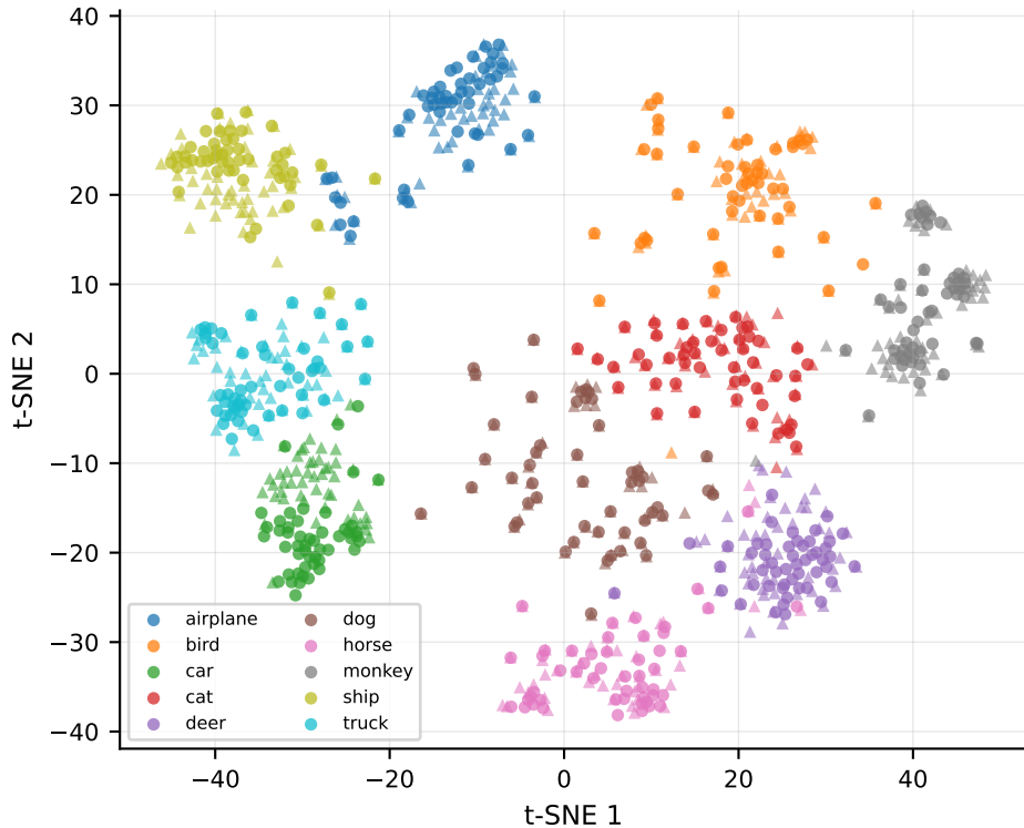
vit_b16 — clean (o) vs patch_shuffle (^) (perplexity=30, metric=cosine, seed=6304)
