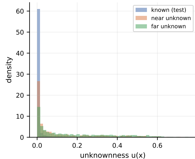
MSP
