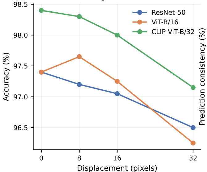
Accuracy vs translation
