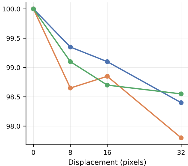
Prediction consistency vs translation
