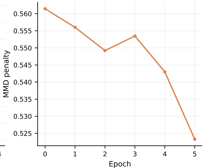
MMD penalty
