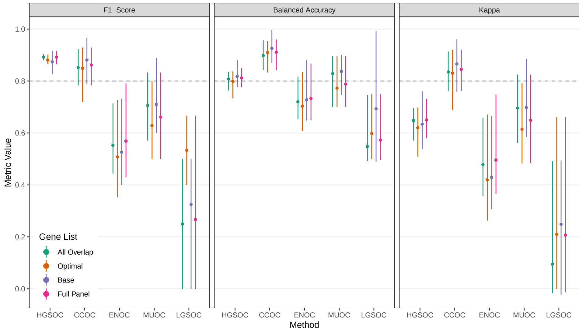
SMOTE-SVM Gene Lists Per-Class Evaluation Metrics by Metric
