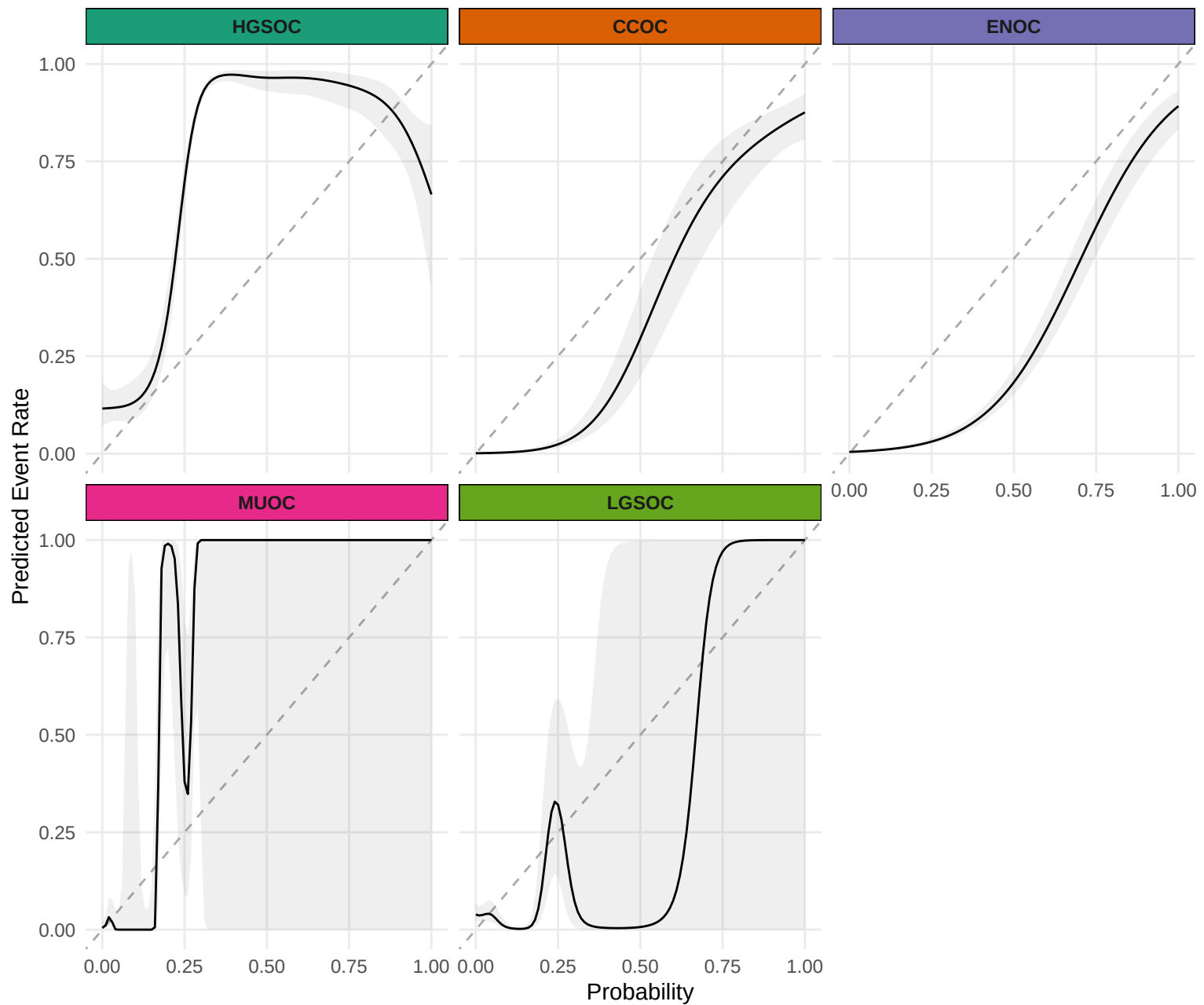
Calibration Plots for SMOTE-SVM, Optimal Set Model in Validation Set
