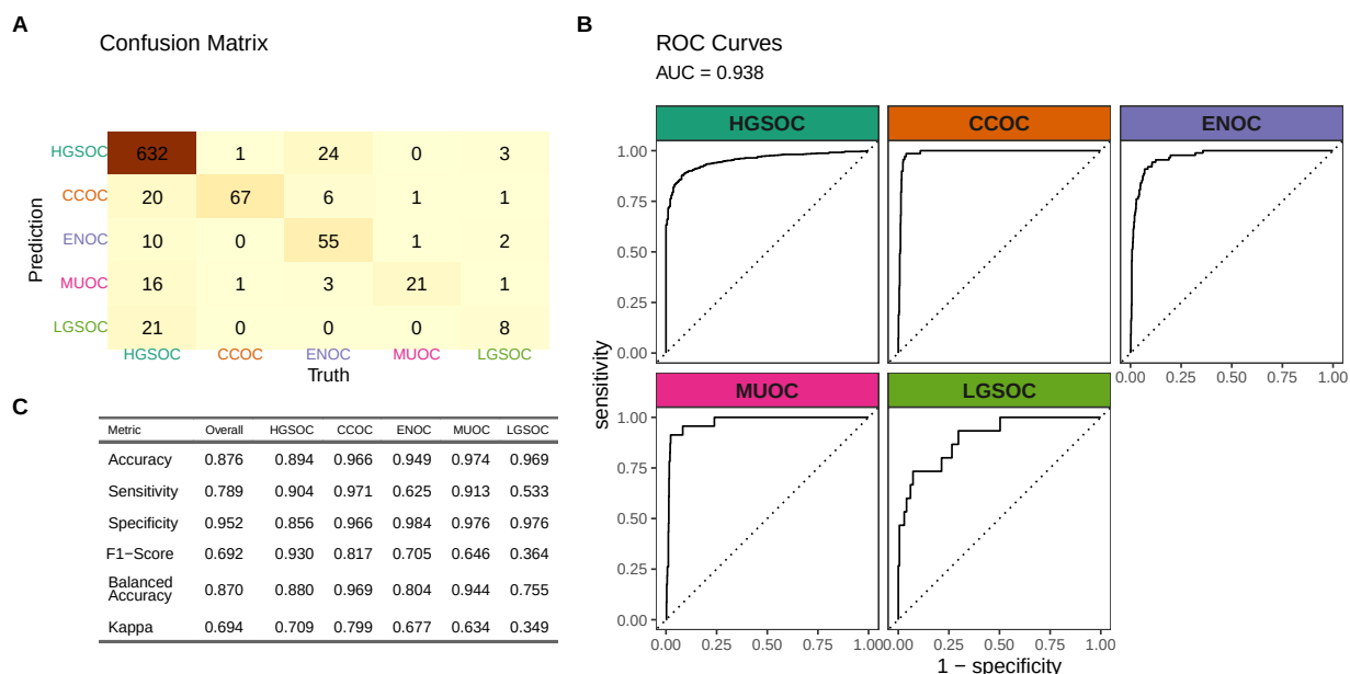
Figure 4.29: Validation Summary
