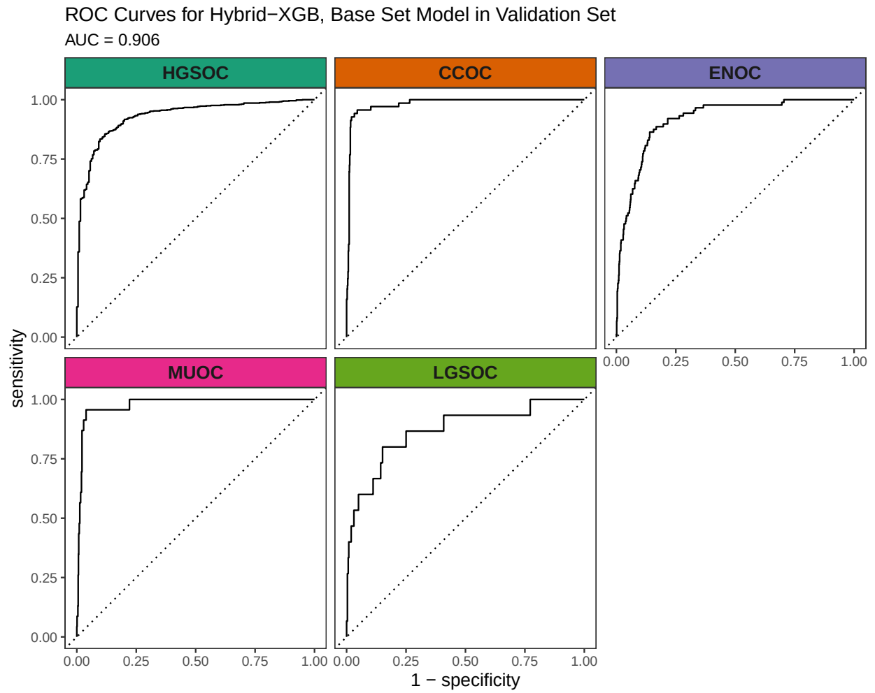
Figure 4.25: ROC Curves for Hybrid-XGB, Base Set Model in Validation Set
