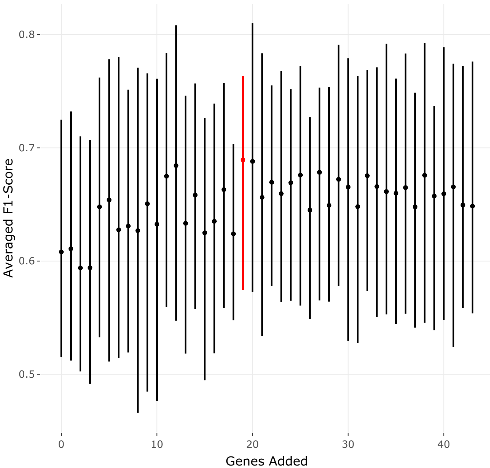
Gene Optimziation for Hybrid-XGB
