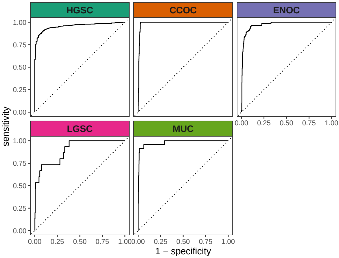
ROC Curve for Up-XGB, Full Set Model in Validation Set AUC = 0.932
