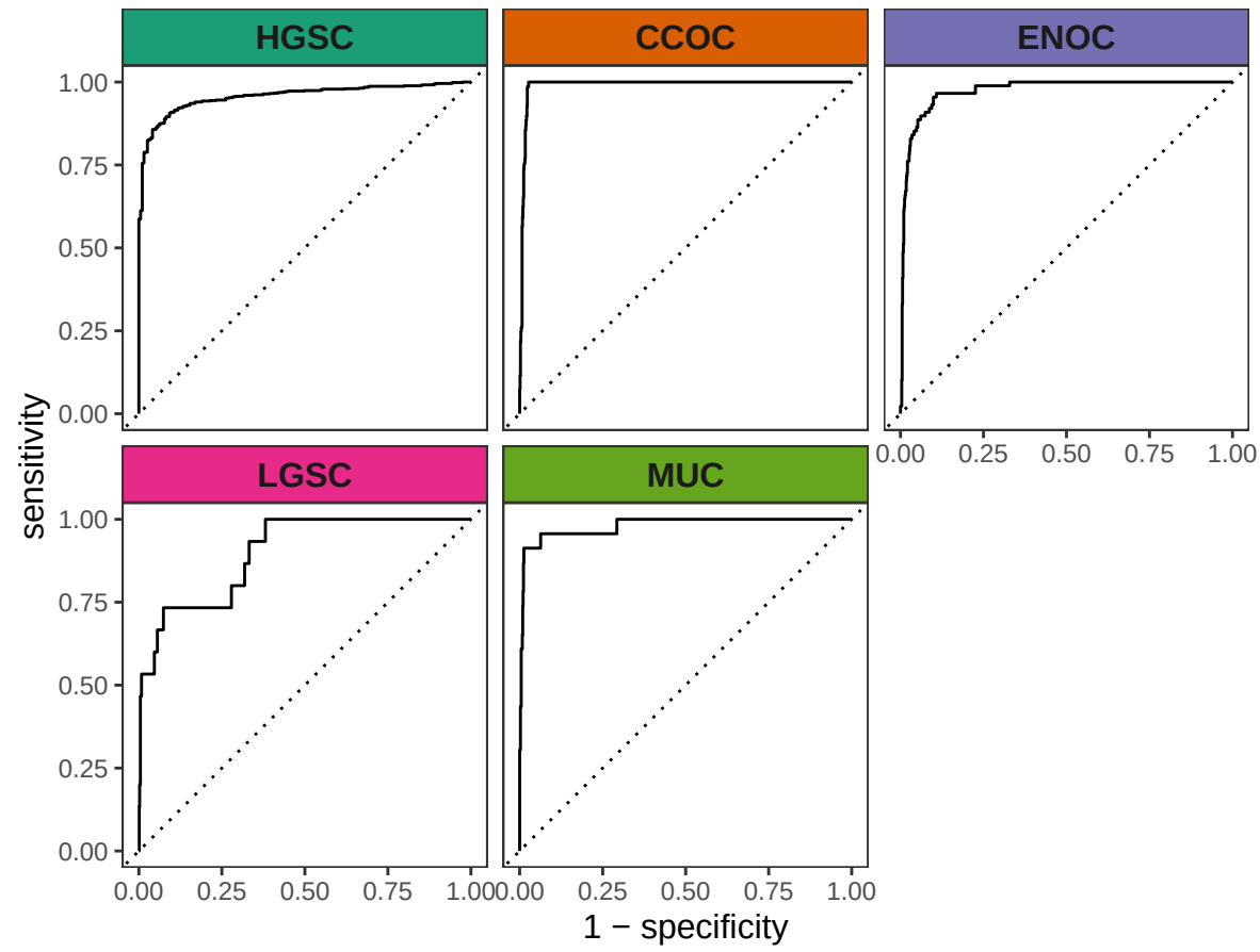
ROC Curve for Up-XGB, Full Set Model in Validation Set AUC = 0.932
