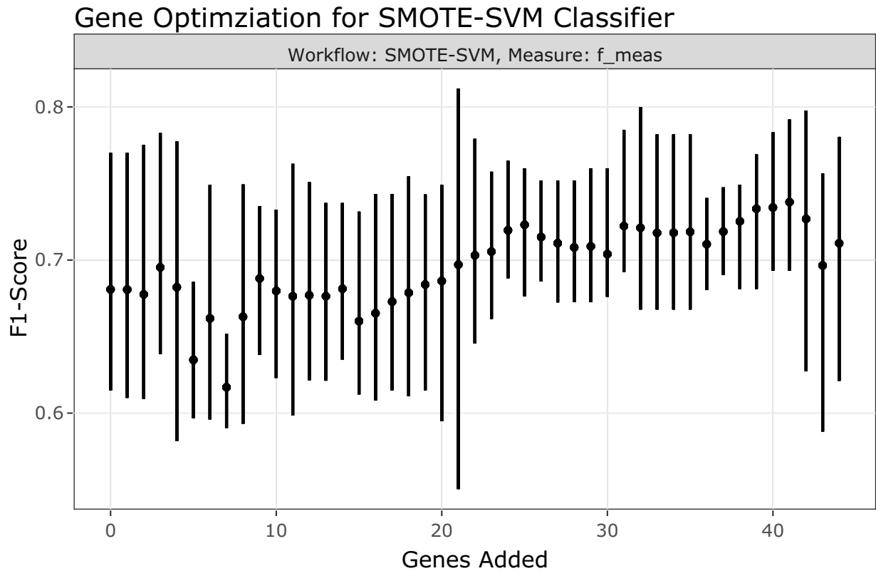
Figure 4.18: Gene Optimization for SMOTE-SVM Classifier
