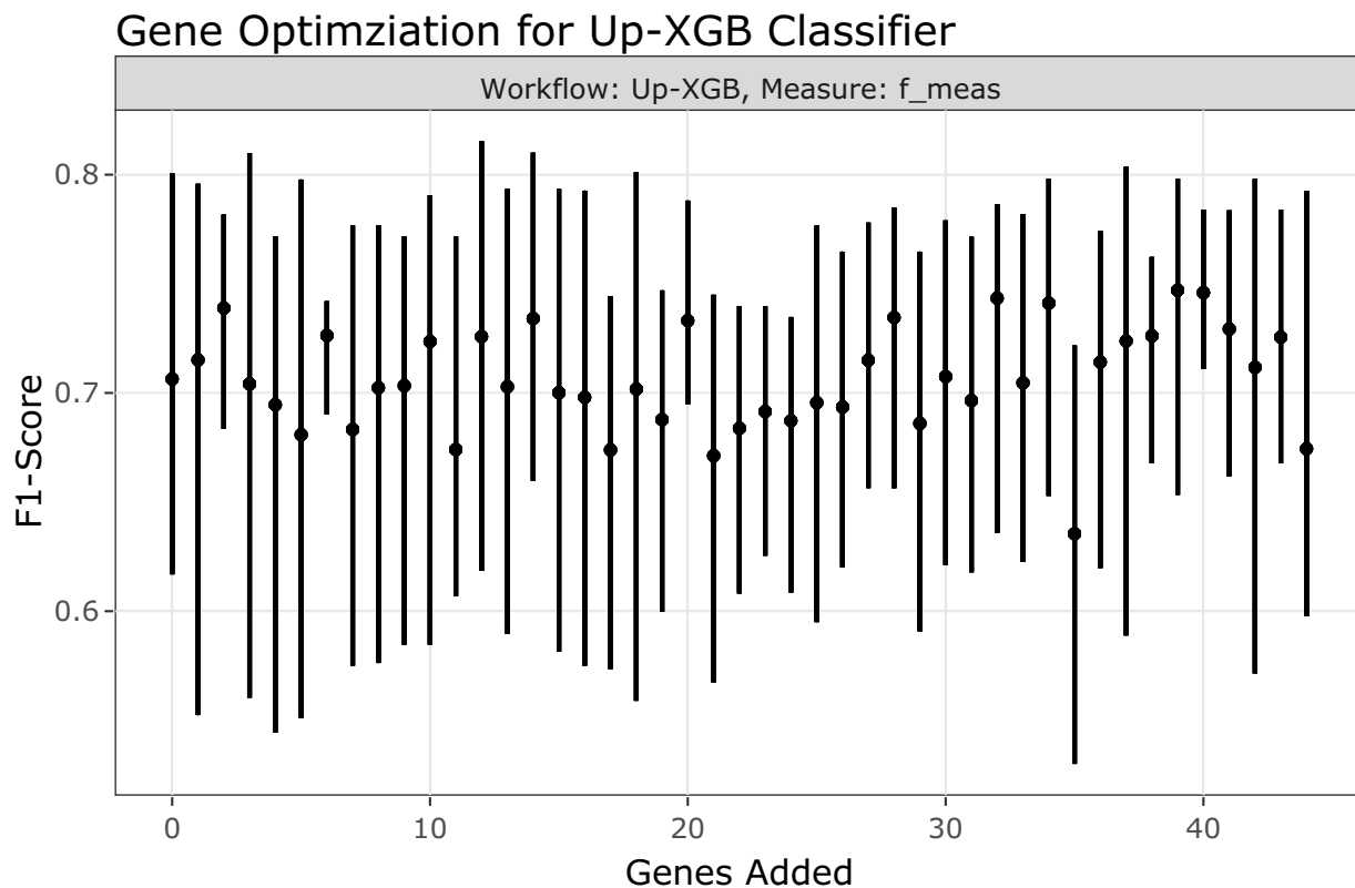
Figure 4.17: Gene Optimization for Up-XGB Classifier
