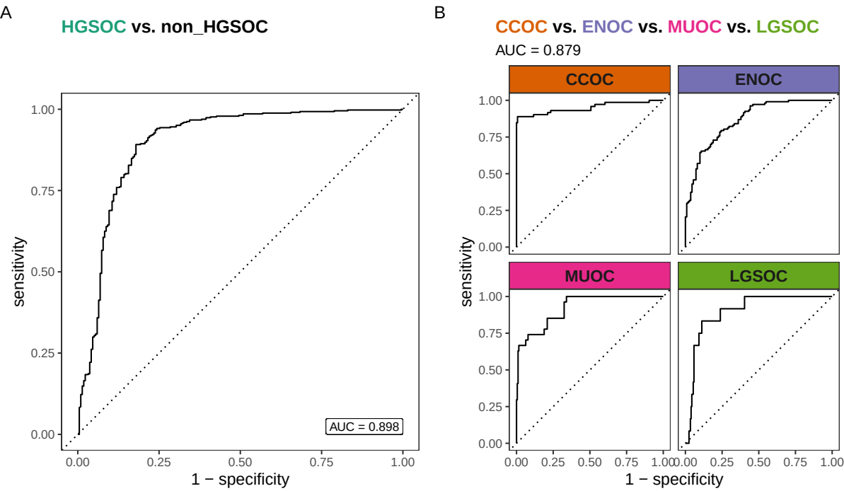
ROC Curves for 2-STEP Model in Confirmation Set
