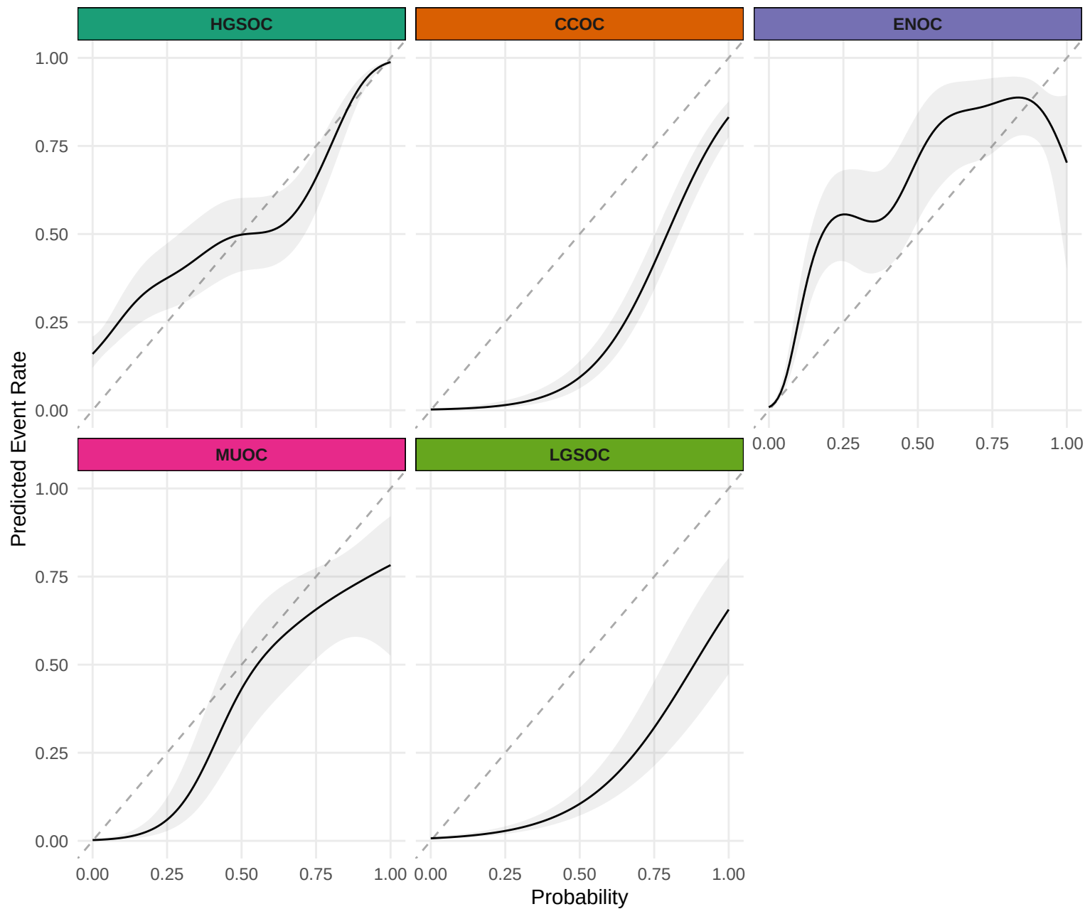
Calibration Plots for Up-XGB, Optimal Set Model in Validation Set
