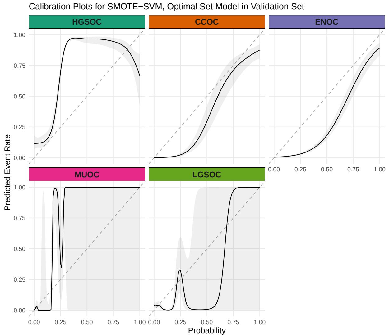
Figure 4.26: Calibration Plots for SMOTE-SVM, Optimal Set Model in Validation Set
