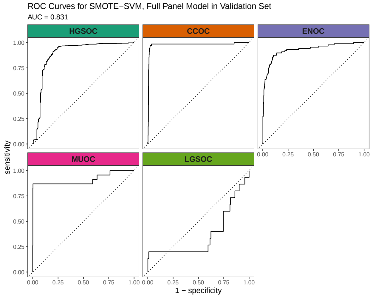
Figure 4.24: ROC Curves for SMOTE-SVM, Full Panel Model in Validation Set
