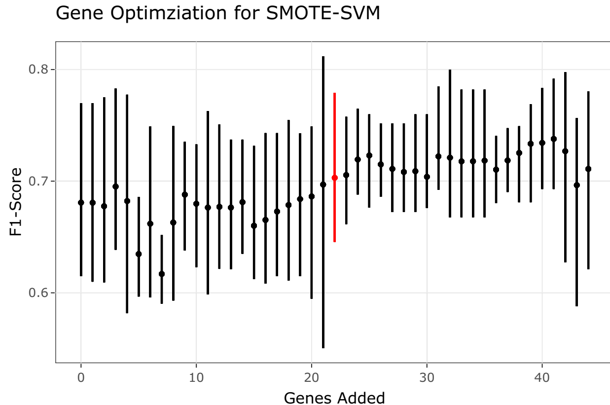
Figure 4.18: Gene Optimization for SMOTE-SVM Classifier using F1-Score
