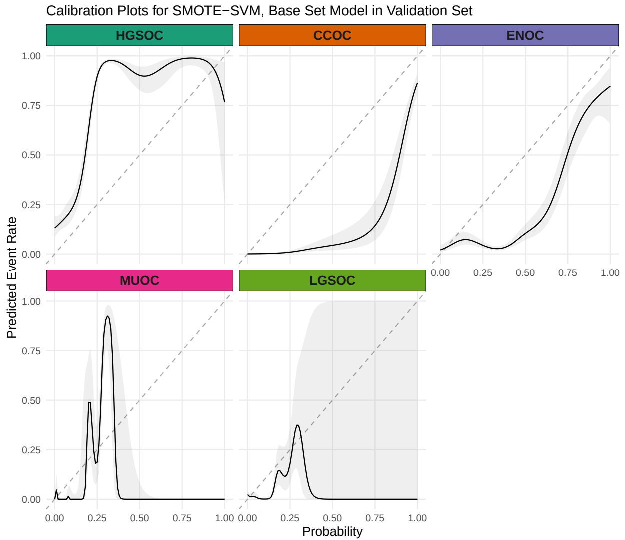
Figure 4.27: Calibration Plots for SMOTE-SVM, Base Set Model in Validation Set
