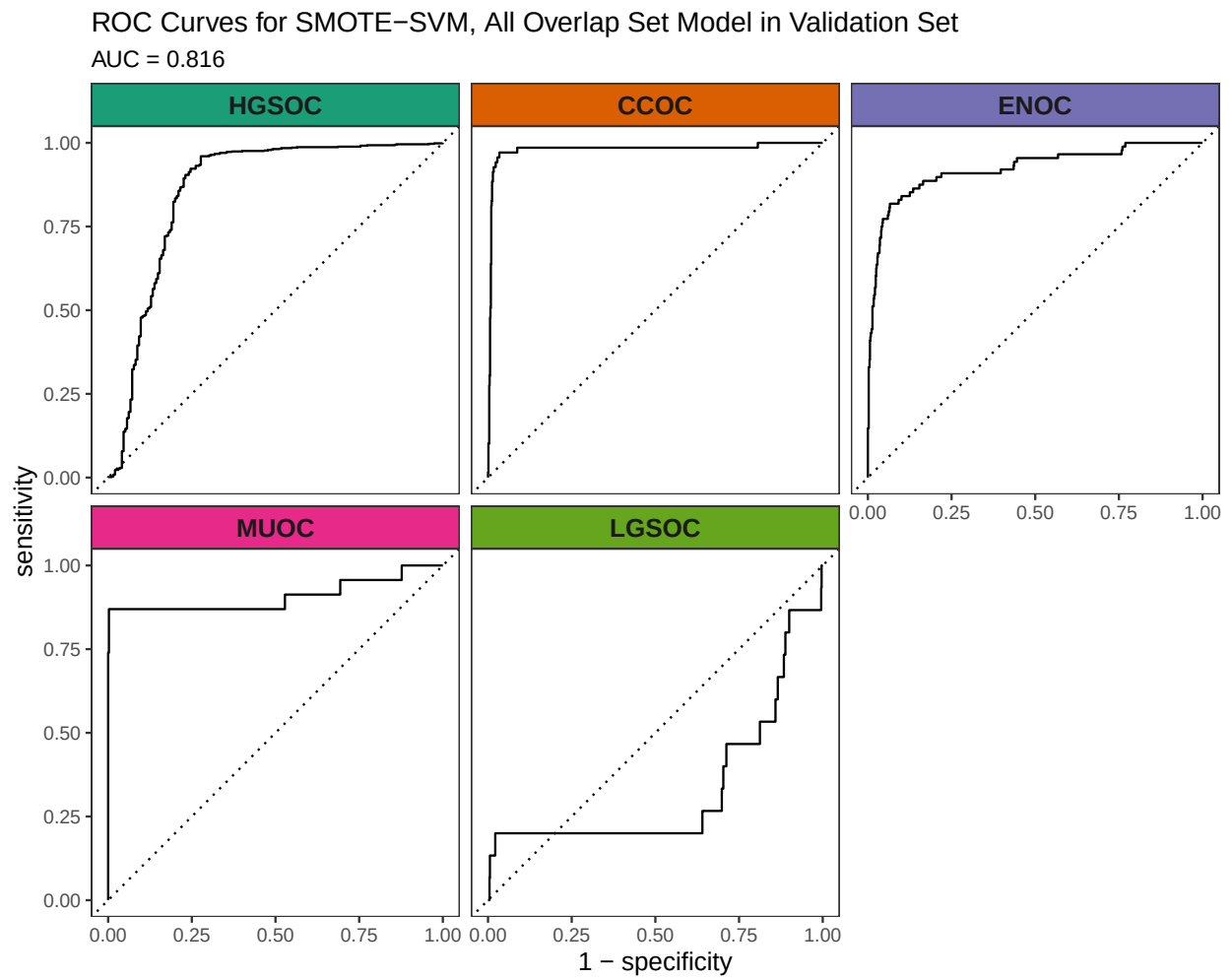
Figure 4.21: ROC Curves for SMOTE-SVM, All Overlap Set Model in Validation Set
