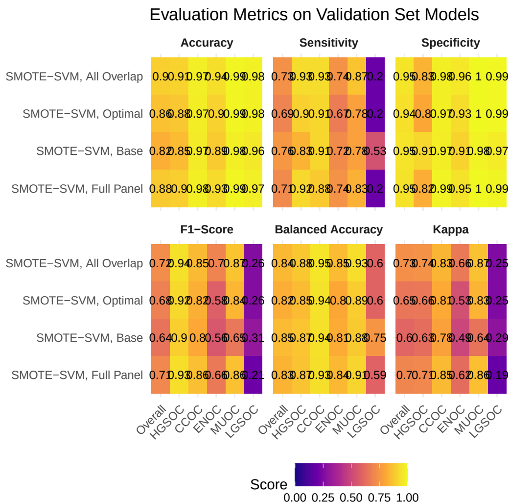
Figure 4.19: Evaluation Metrics on Validation Set Models
