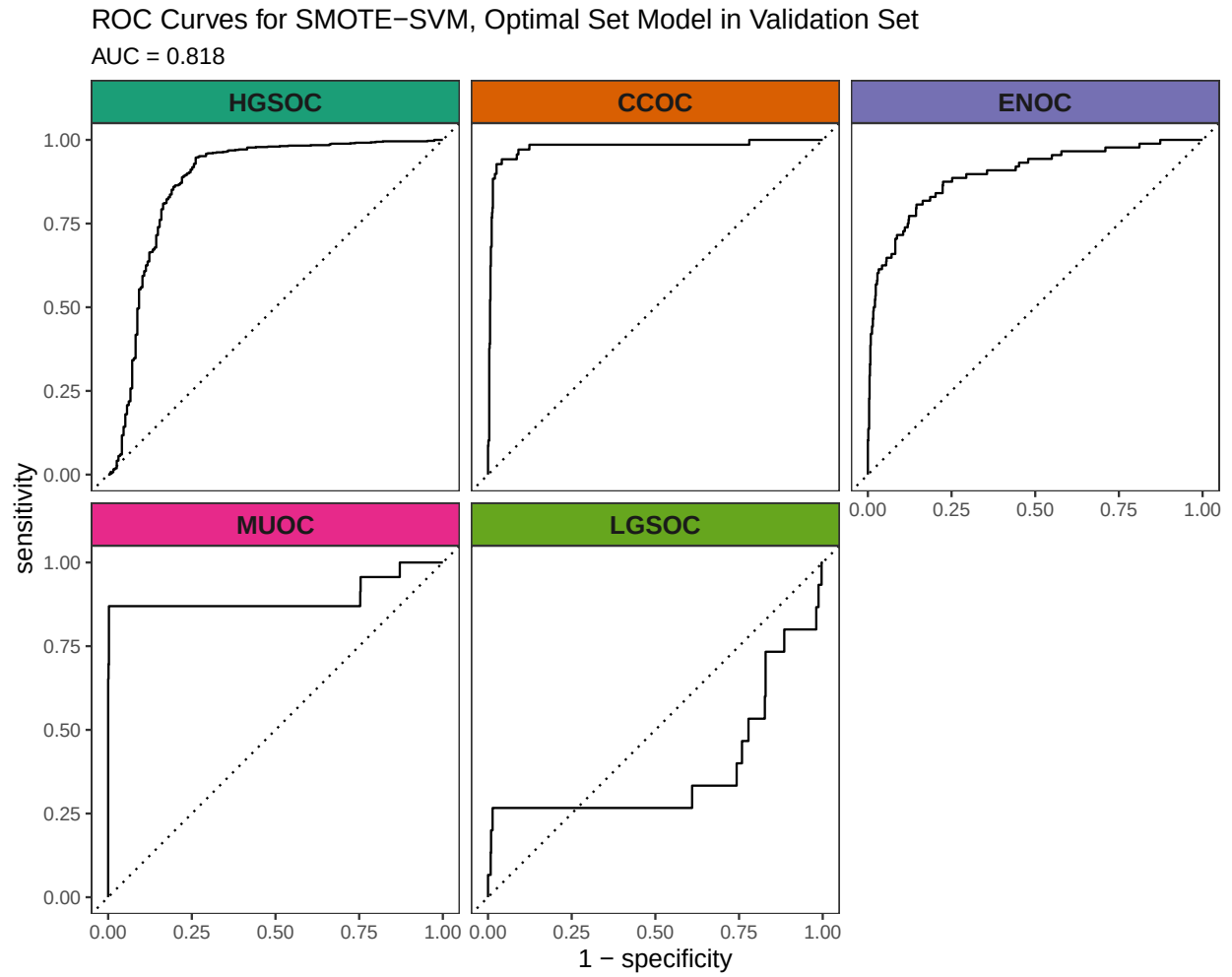
Figure 4.22: ROC Curves for SMOTE-SVM, Optimal Set Model in Validation Set
