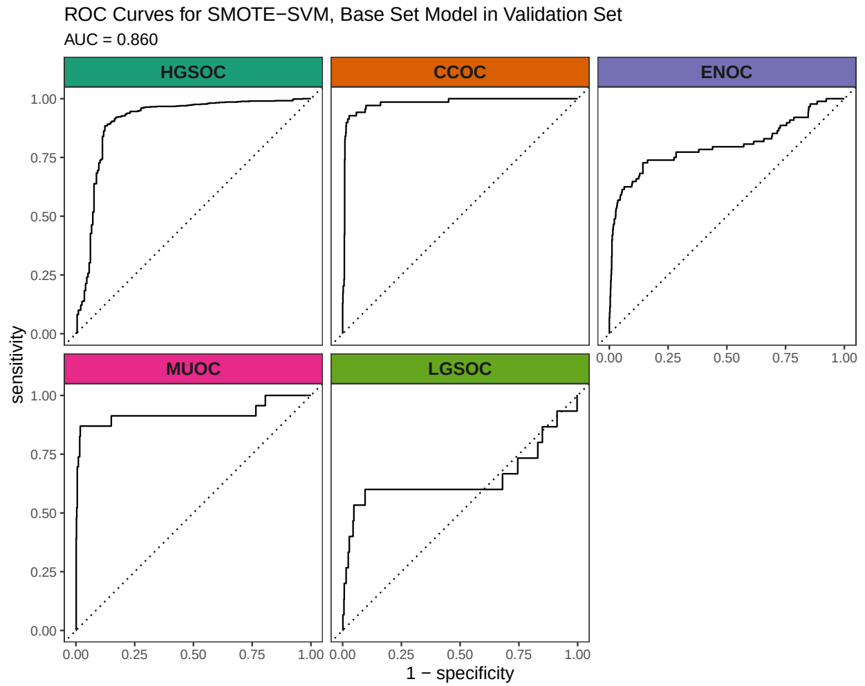
Figure 4.23: ROC Curves for SMOTE-SVM, Base Set Model in Validation Set
