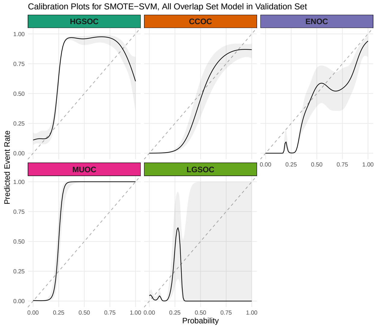
Figure 4.25: Calibration Plots for SMOTE-SVM, All Overlap Set Model in Validation Set
