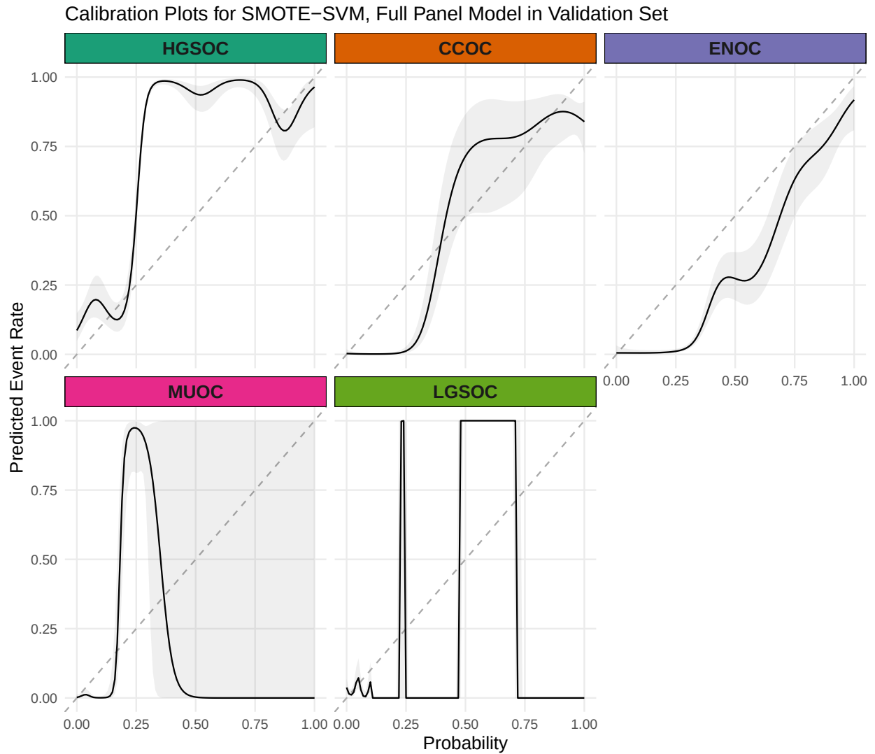
Figure 4.28: Calibration Plots for SMOTE-SVM, Full Panel Model in Validation Set
