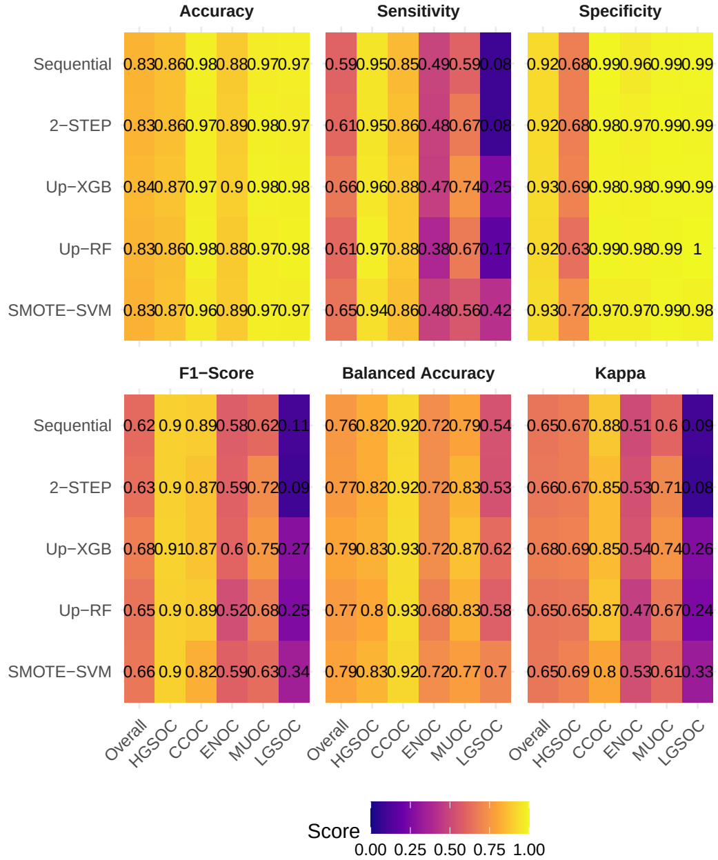
Evaluation Metrics on Confirmation Set Models
