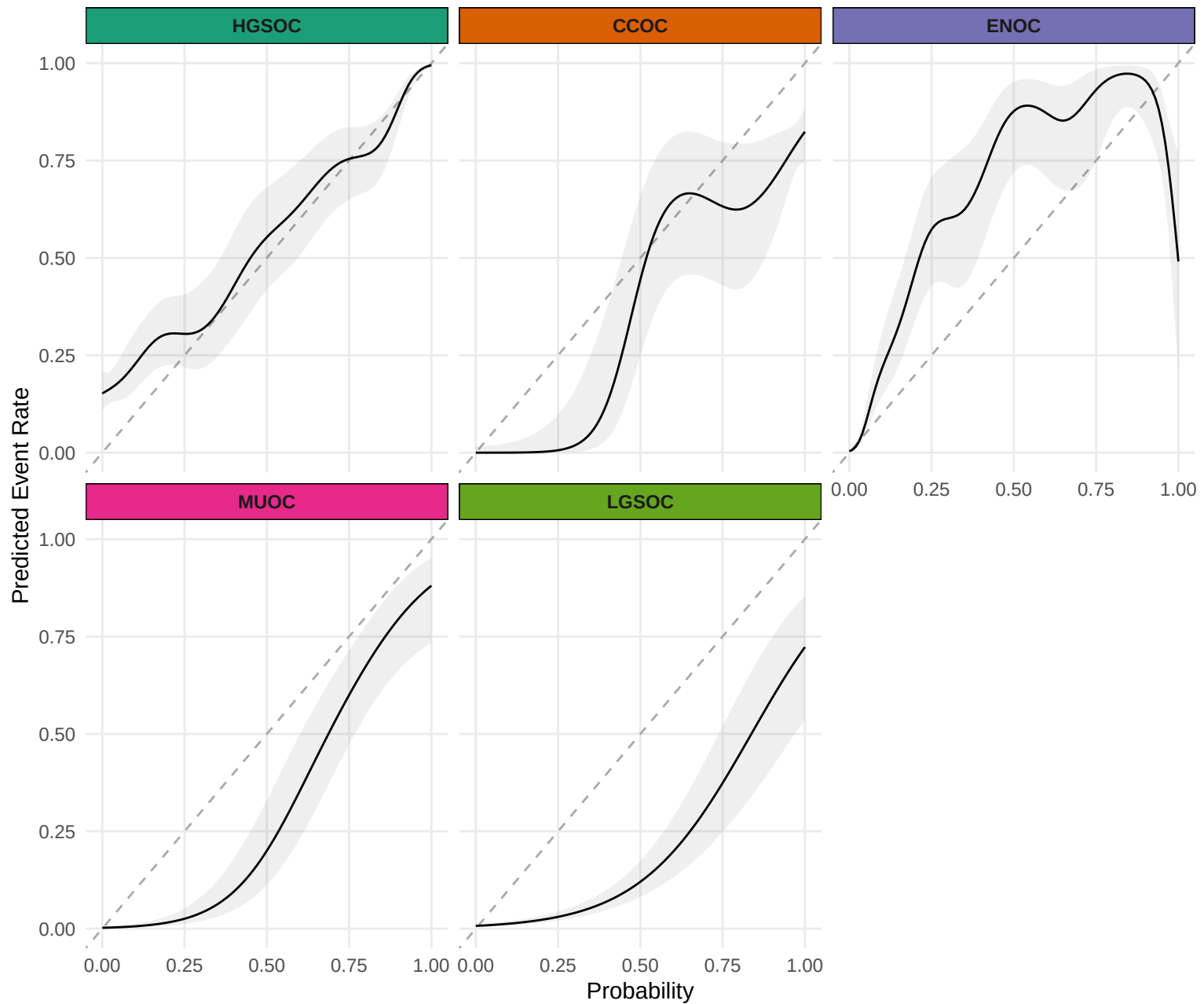
Calibration Plots for Up-XGB, Full Set Model in Validation Set
