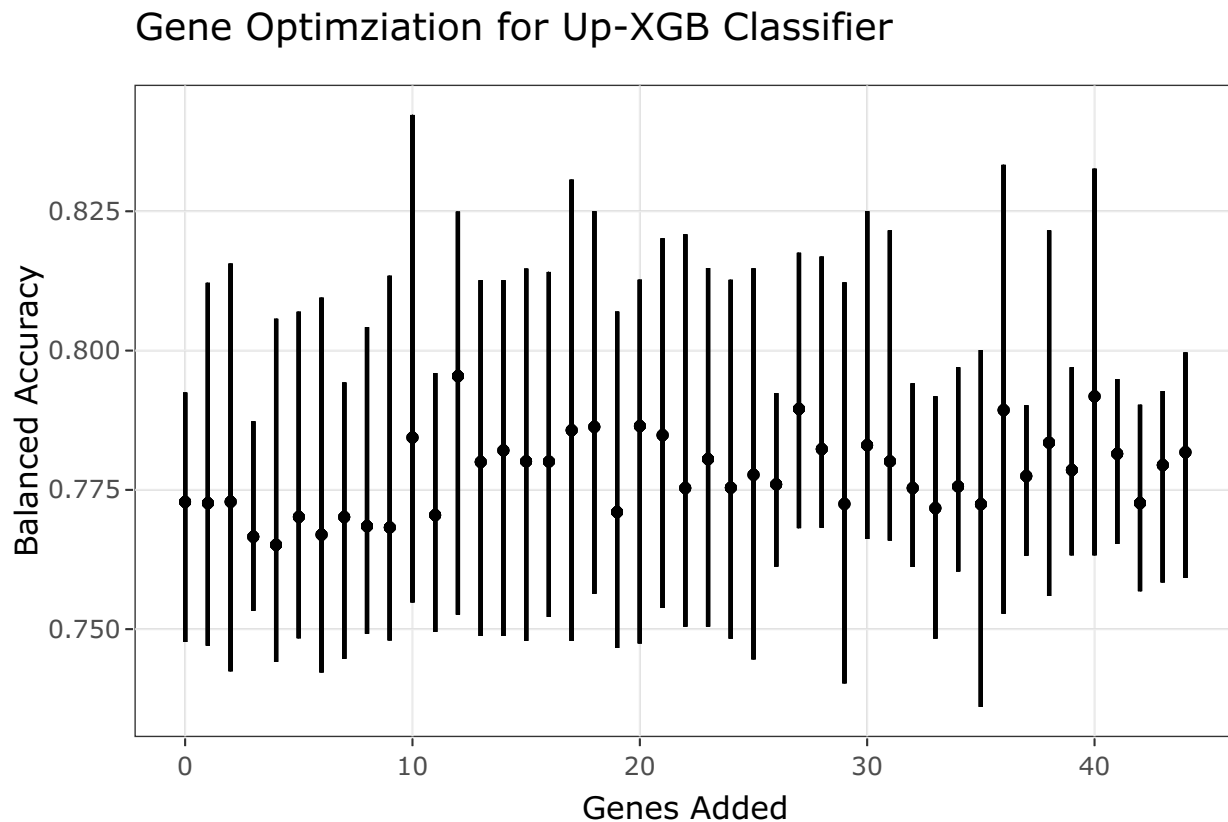
Figure 4.18: Gene Optimization for Up-XGB Classifier using Balanced Accuracy
