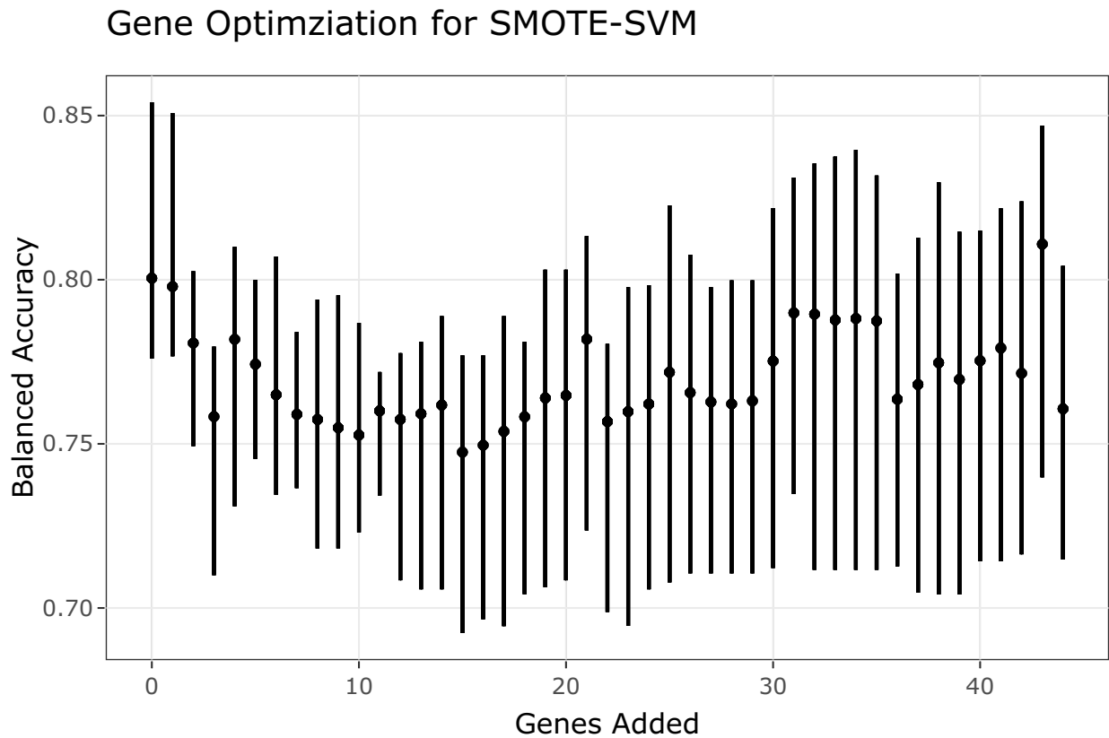
Figure 4.19: Gene Optimization for SMOTE-SVM Classifier using Balanced Accuracy
