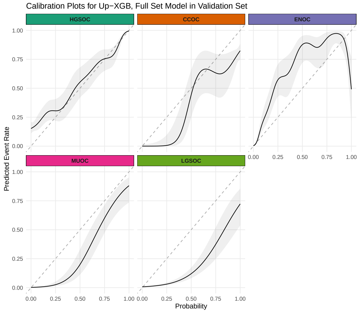
Figure 4.23: Calibration Plots for Up-XGB, Full Set Model in Validation Set
