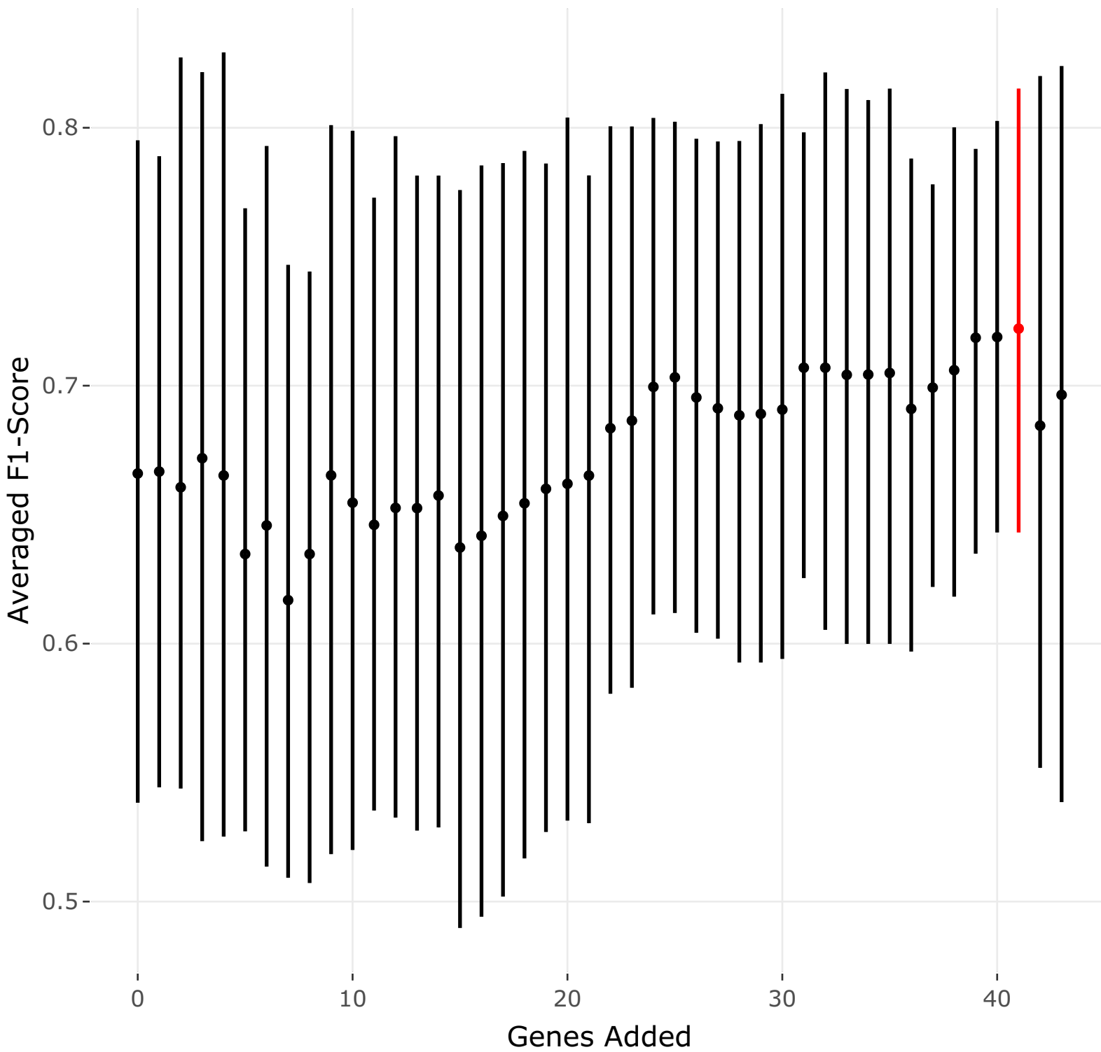
Gene Optimziation for SMOTE-SVM
