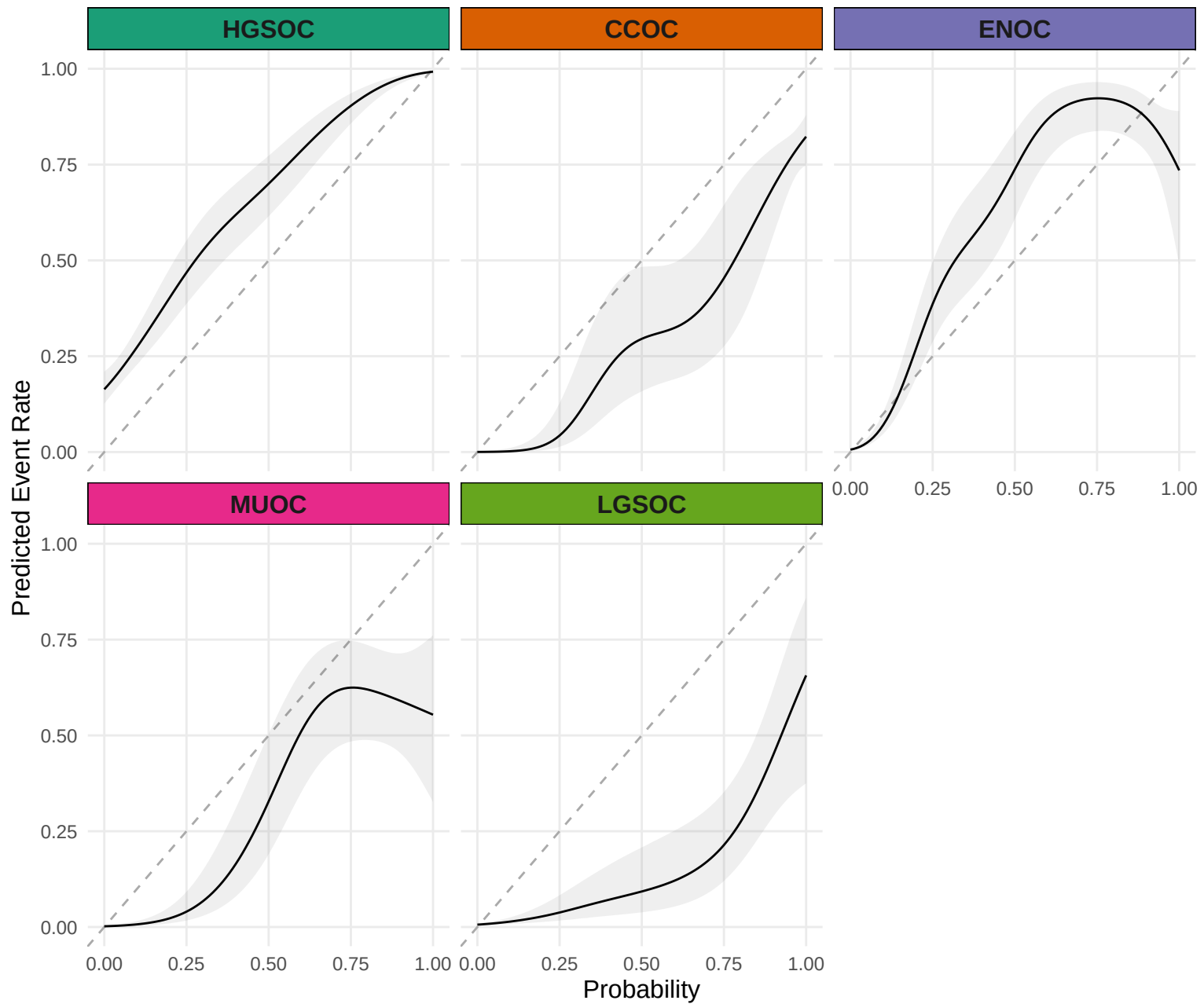
Calibration Plots for Hybrid-XGB, All Overlap Set Model in Validation Set
