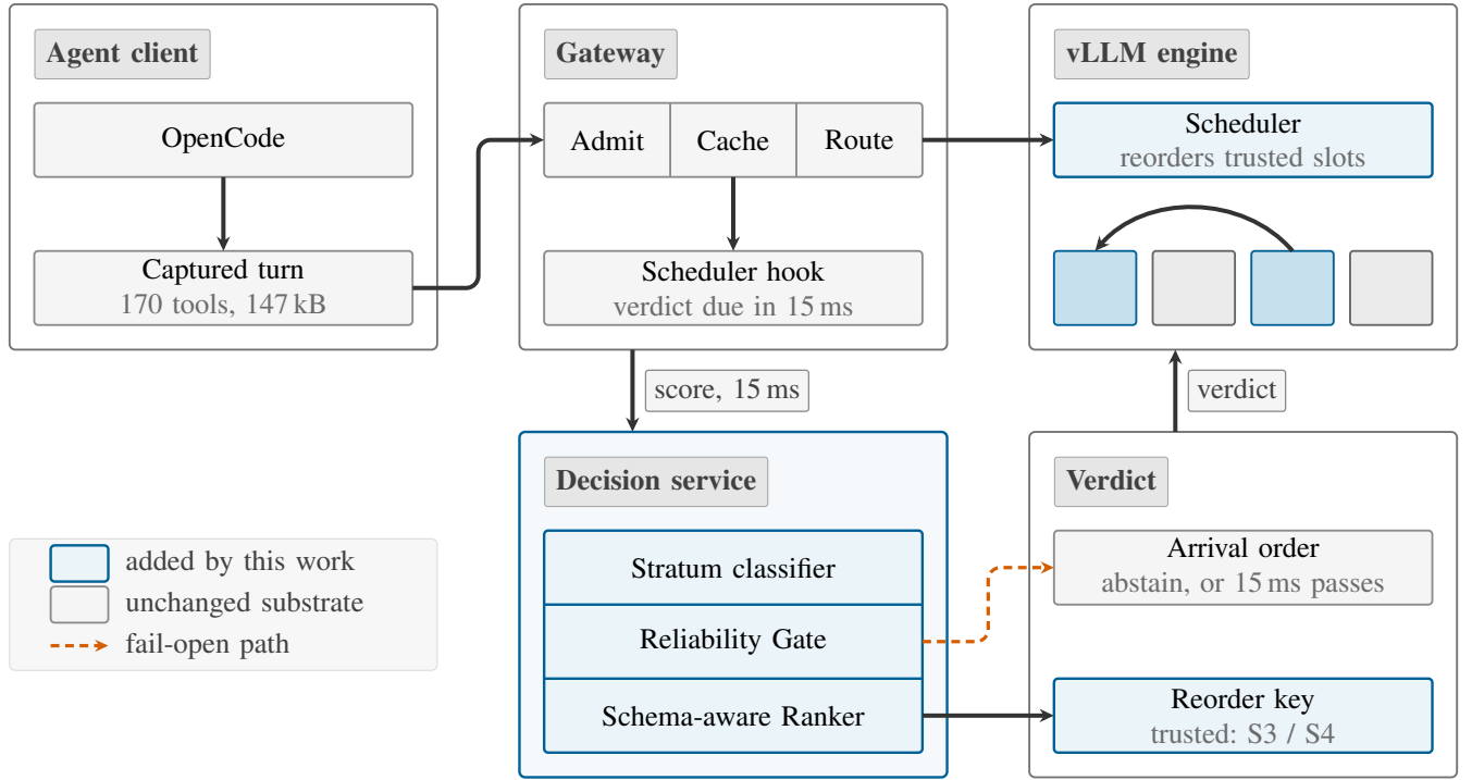
Fig. 1. The gateway scores at admission inside a 15 ms budget and forwards the verdict; the engine’s scheduler reorders trusted slots among themselves and leaves abstained ones where they arrived. A timeout or an abstention yields arrival order.
