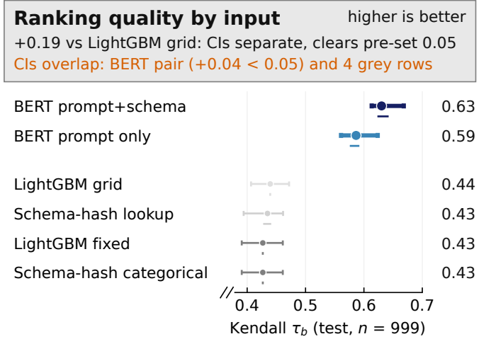
Fig. 4. Ranking quality by input family: prompt-plus-schema text exceeds the tuned scalar baseline by \Delta\tau_b = +0.191 . Dots are the mean over 3 seeds; capped bars the 95% bootstrap CI on seed 17 alone; the lane below each row the min–max across seeds, a tick where that spread is zero.
