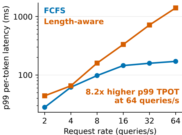
Tail per-token cost (lower is better)
