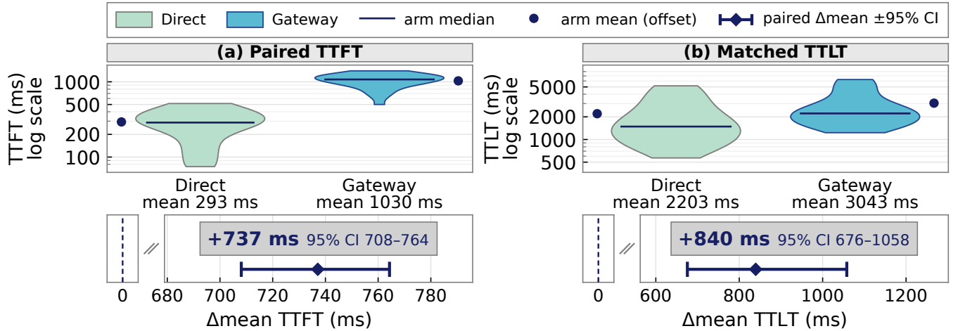
Fig. 6. Admission-time scoring versus direct: +737 ms TTFT and +840 ms TTLT over the whole added path. Panel (a) is 150 paired requests and (b) the 118 of them with equal output tokens; violin bodies and y-axes are trimmed to p5–p95 of each arm, and intervals are 2,000\times bootstrap percentile CIs.
