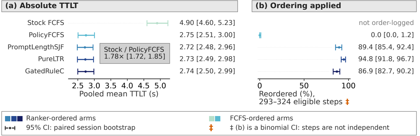
Fig. 9. Serving-level scheduling at the default batch cap: the 1.78× gap between stock and PolicyFCFS comes from the scheduler implementation, not from ordering, and the policies rewrote 87–95% of the steps that could express an order. The paired ordering ratios for this regime, and the 3% margin they are judged against, are in Fig. 8(a).
