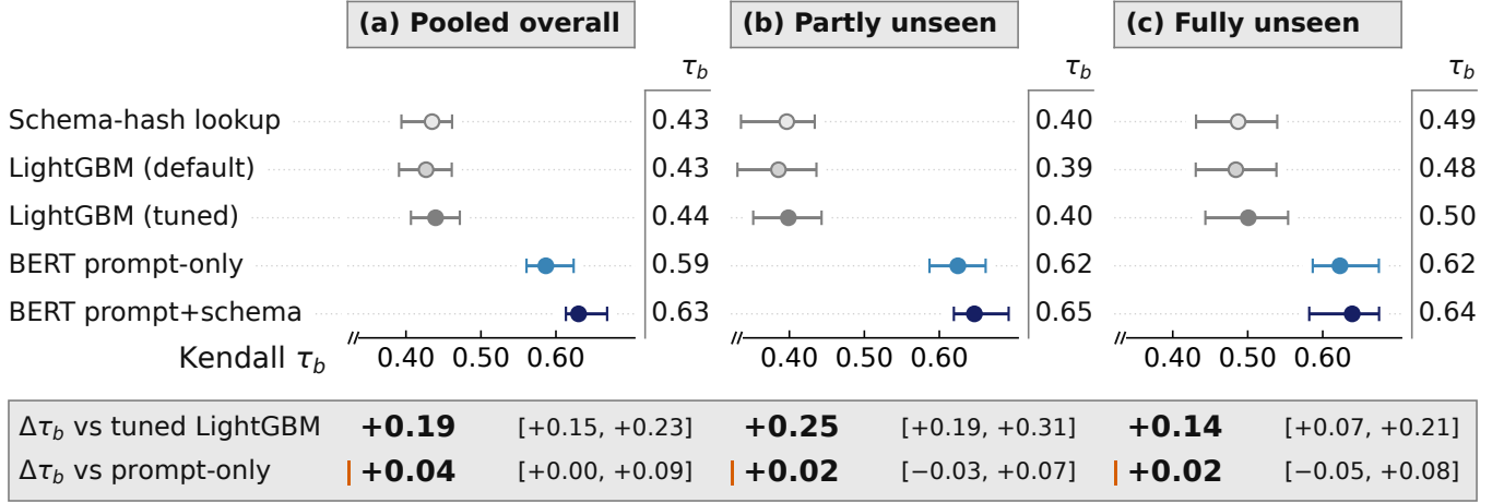
Fig. 5. Cold-start transfer: schema-text ranking differs by 0.0075 between the two adequately powered unseen-tool strata, and the identity lookup records no table hits. Panel (a) pools all 999 test requests, including the withheld S1 and S2 of Fig. 2, so it is not the mean of (b) and (c); markers are the mean over three seeds, whiskers are session-clustered bootstrap CIs (1000 resamples, percentile, seed-17 scores), and each \Delta\tau_b interval adds the two arms' variances as independent, which is conservative for these paired rows.
