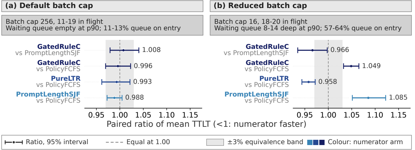
Fig. 8. One engine setting decides the paper’s answer. The same four policies on the same workload: with the default running-batch cap no pair separates, and with the cap reduced every pair does.
