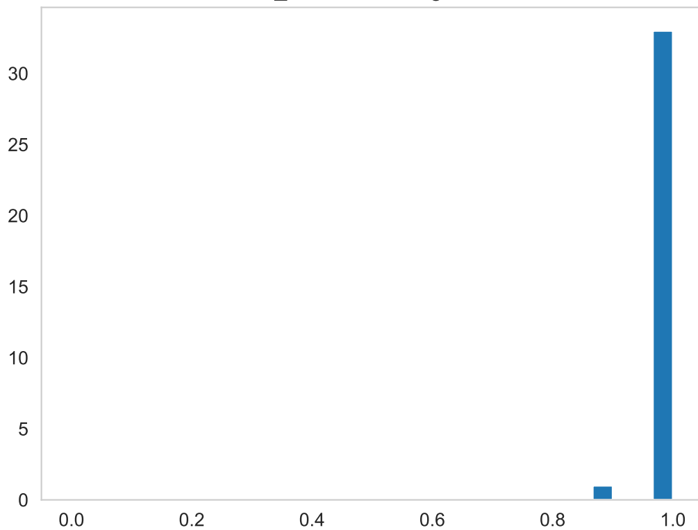
v_measure Histogram
