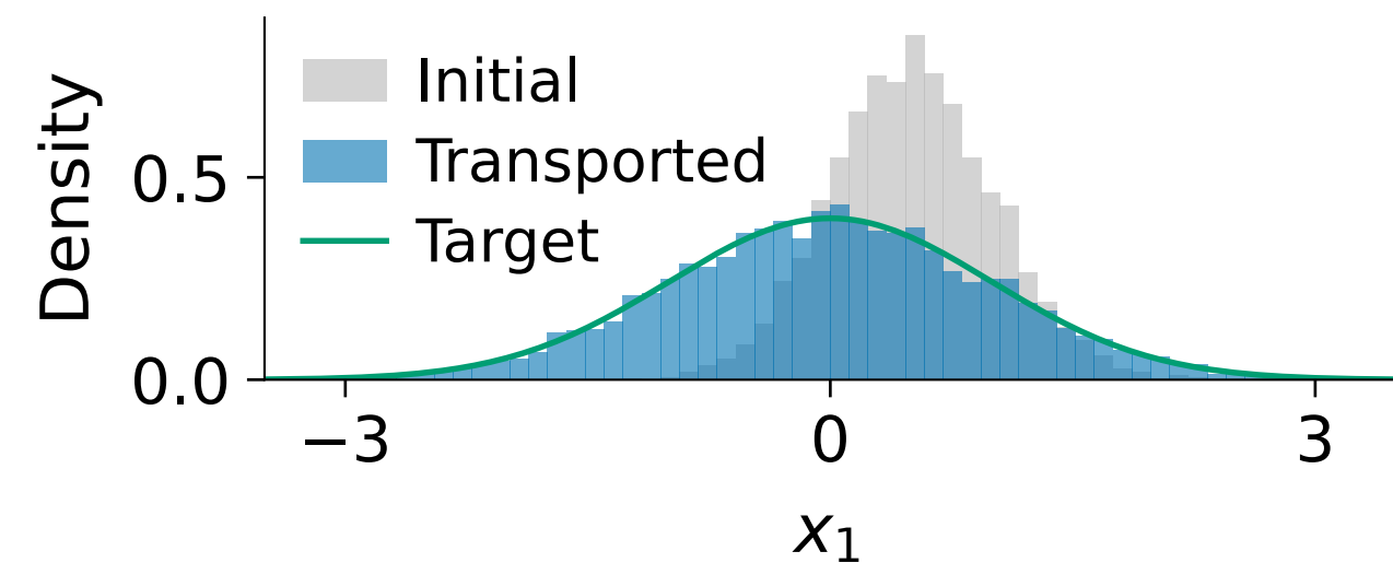
Marginal x_1
