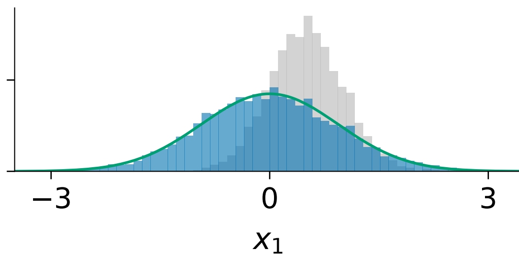
Marginal x_1
