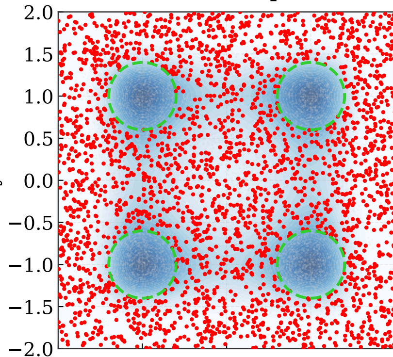
DMPS: step 0
