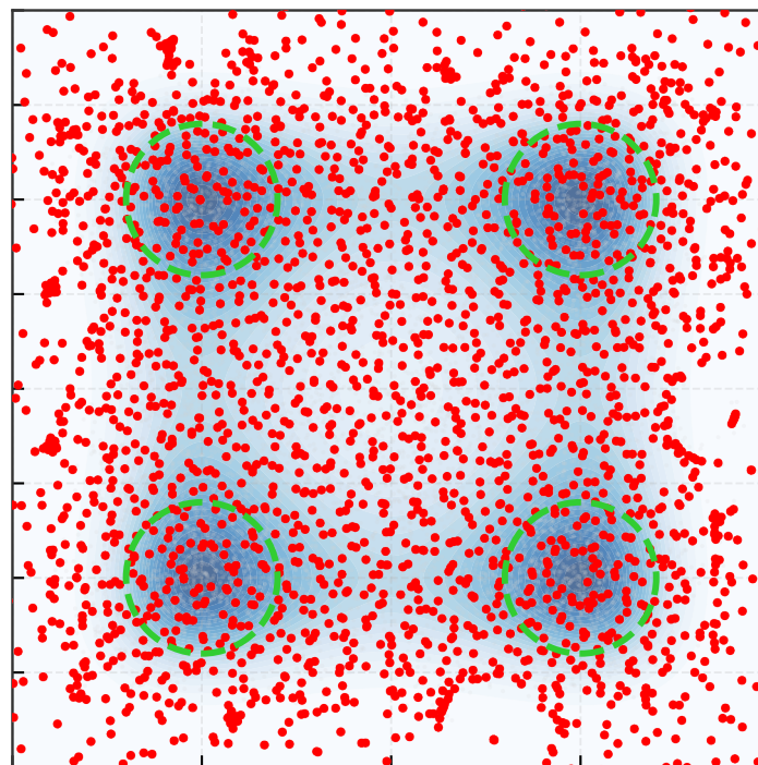
DMPS: step 1000
