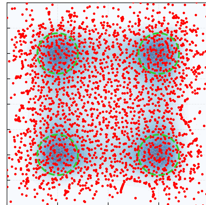
DMPS: step 3000
