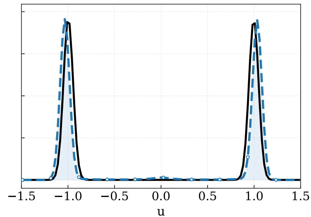
iteration 100
