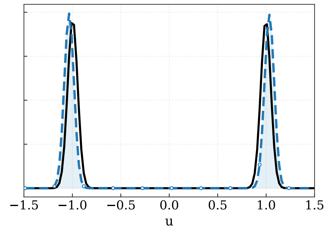
iteration 750
