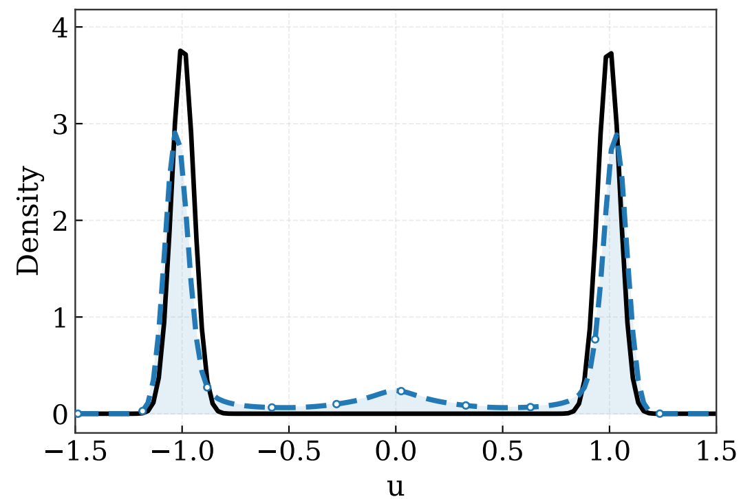
iteration 50
