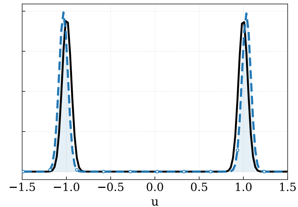
iteration 1500
