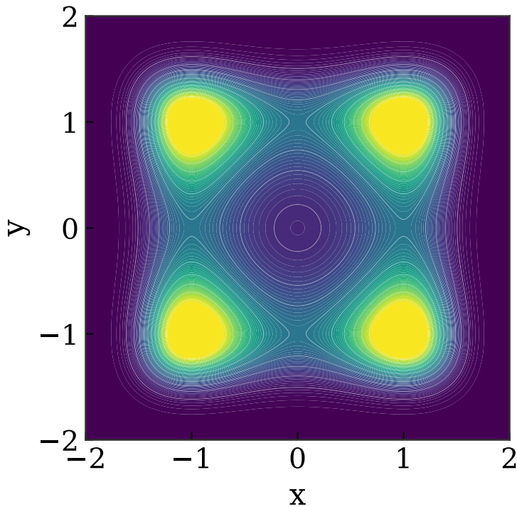
True Boltzmann Distribution
