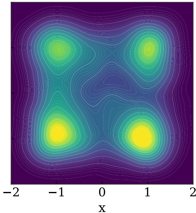
KDE of Training Data
