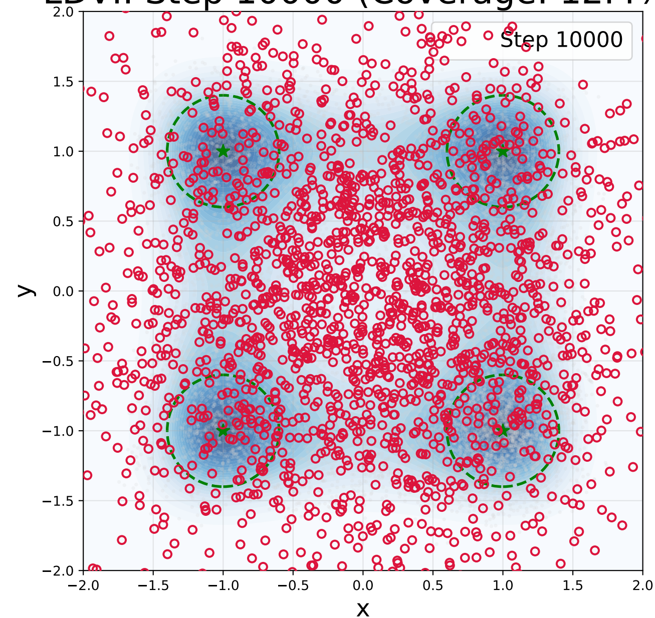
LDVI: Step 10000 (Coverage: 12.4%)
