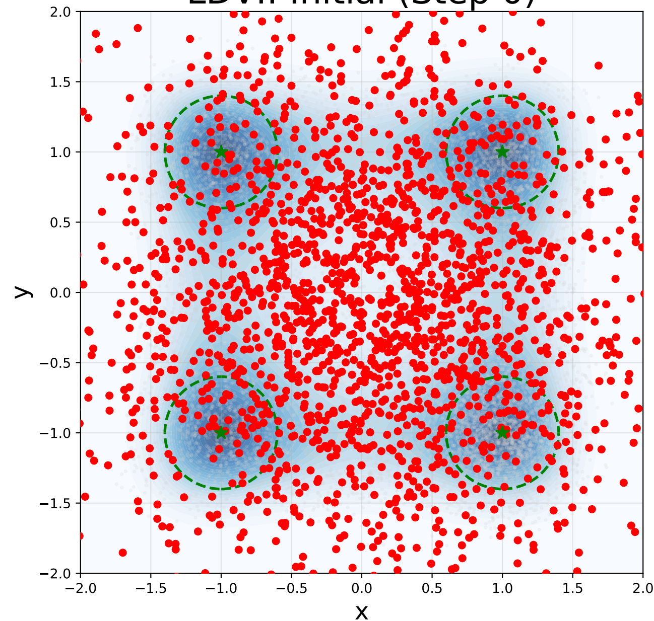
LDVI: Initial (Step 0)
