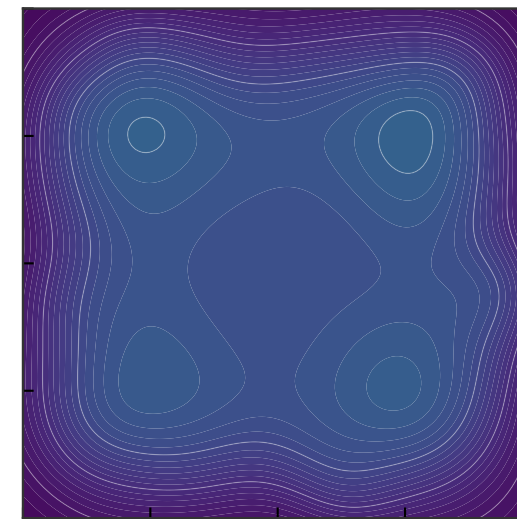
DMPS
