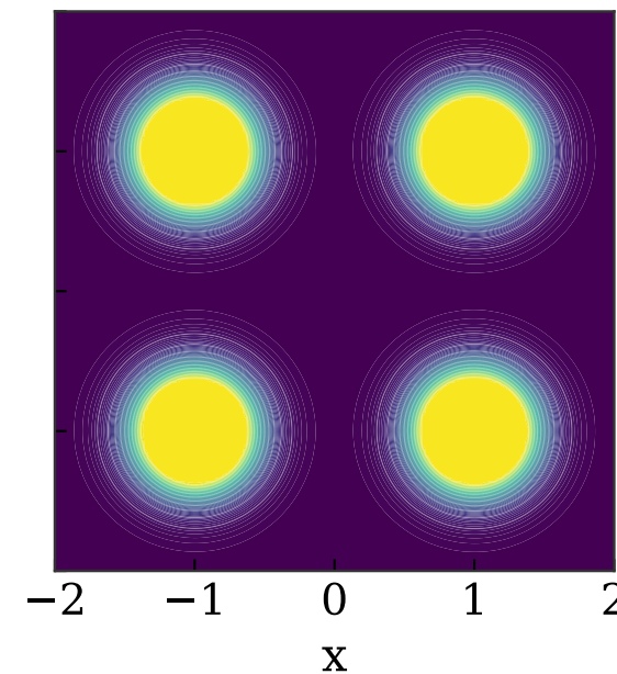
LDVI
