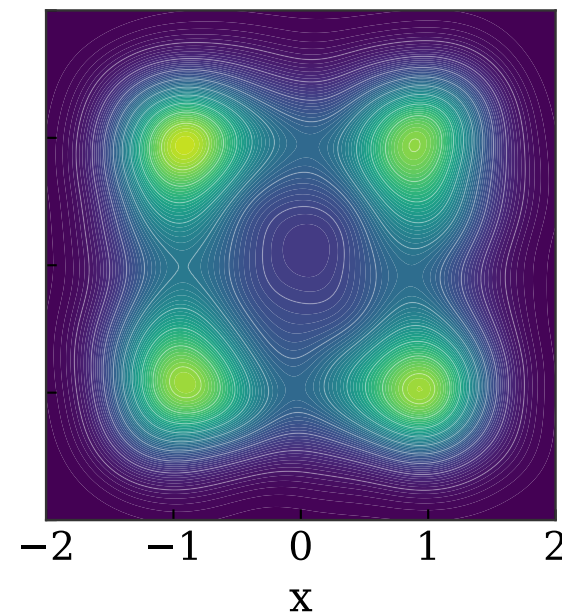
HMC
