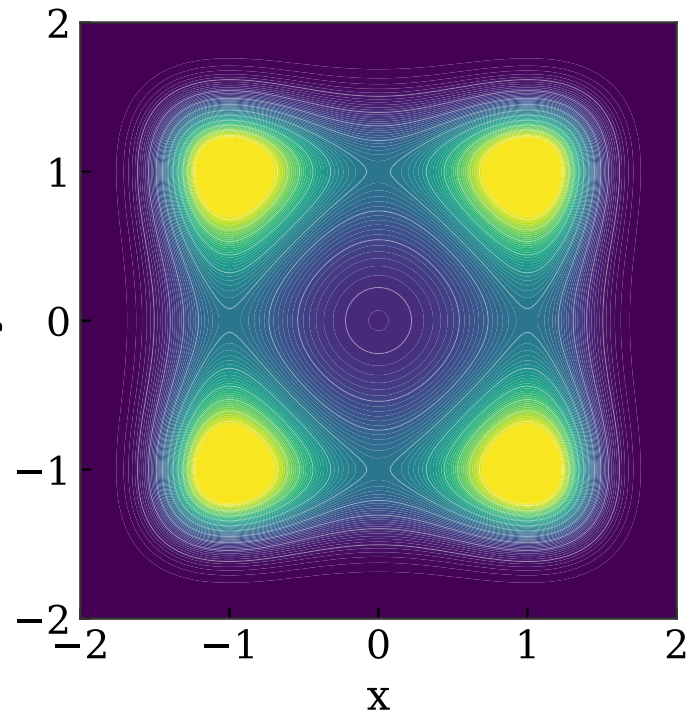
True Boltzmann Distribution
