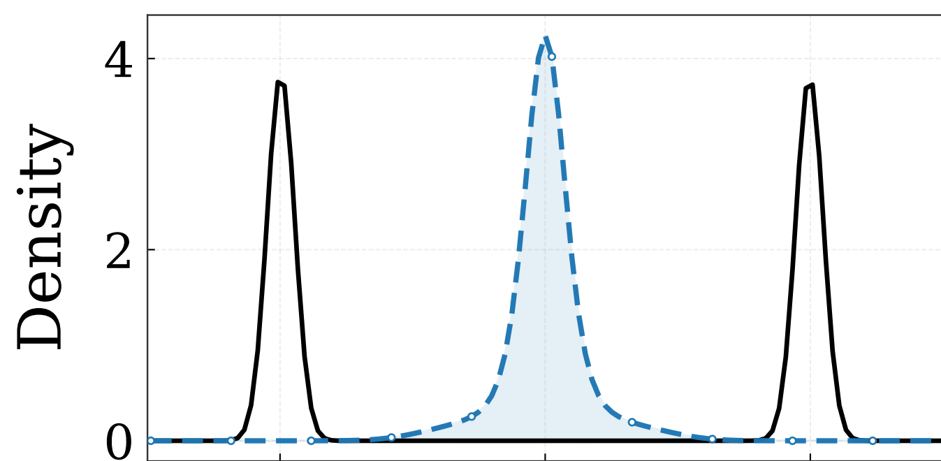
iteration 0
