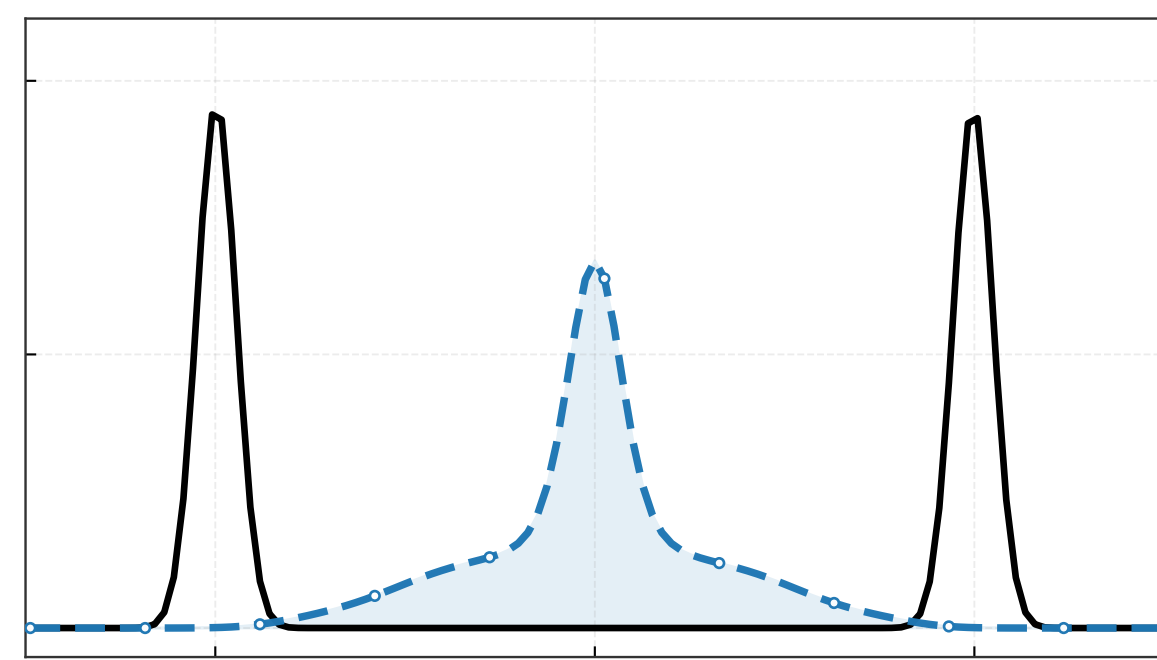
iteration 10
