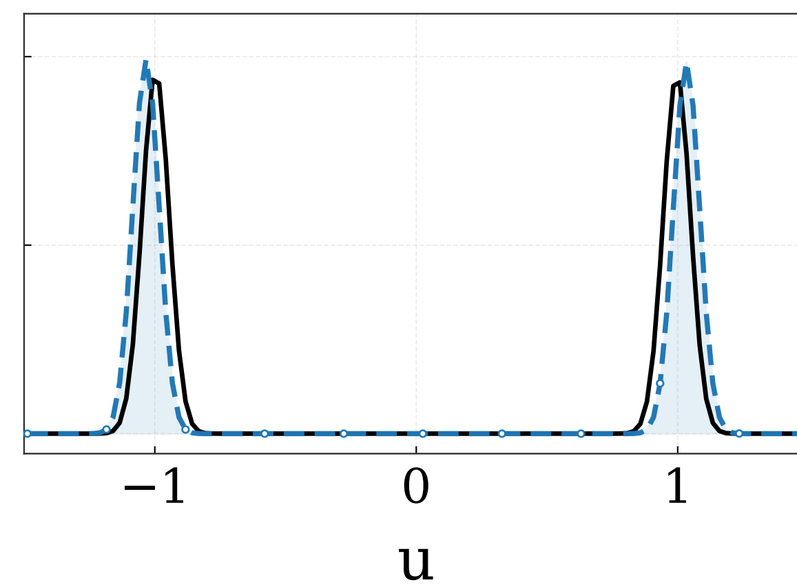
iteration 750
