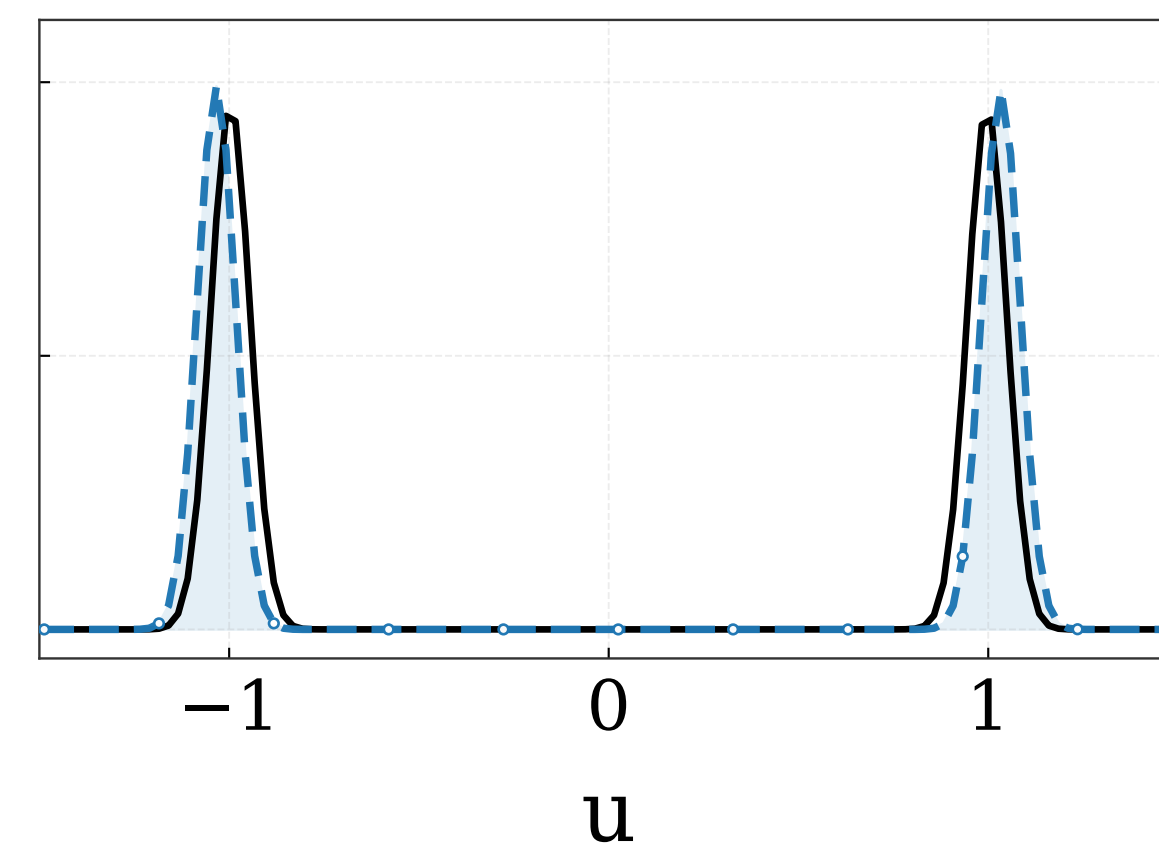
iteration 1500
