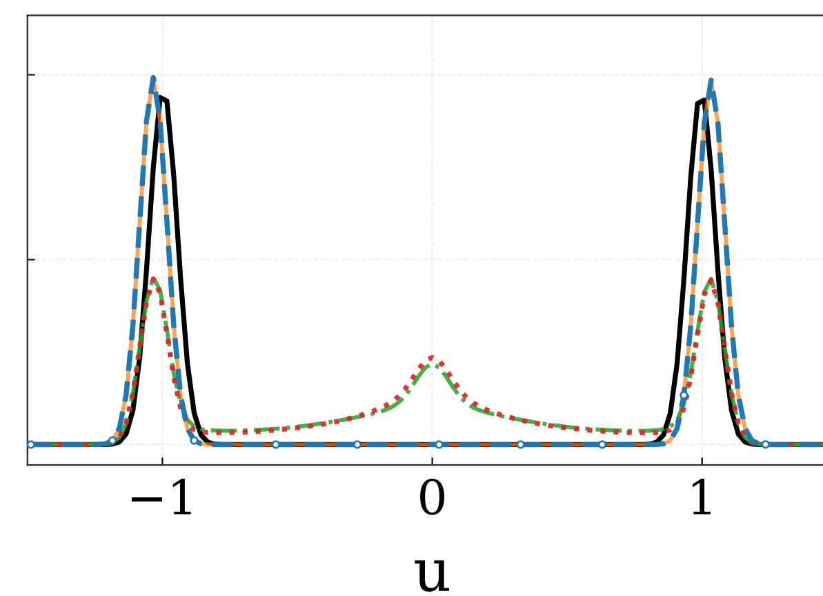
iteration 1500
