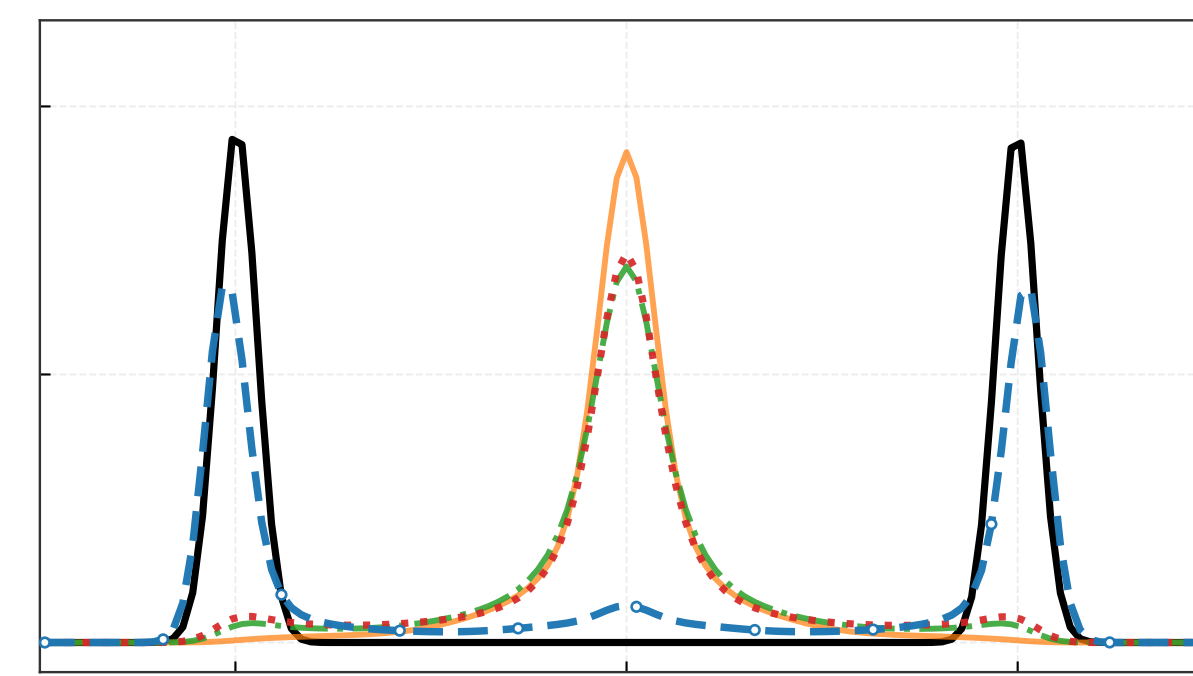
iteration 30
