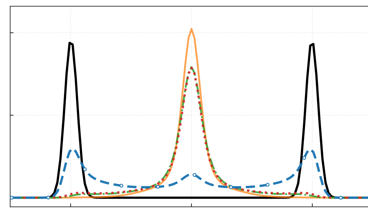
iteration 20
