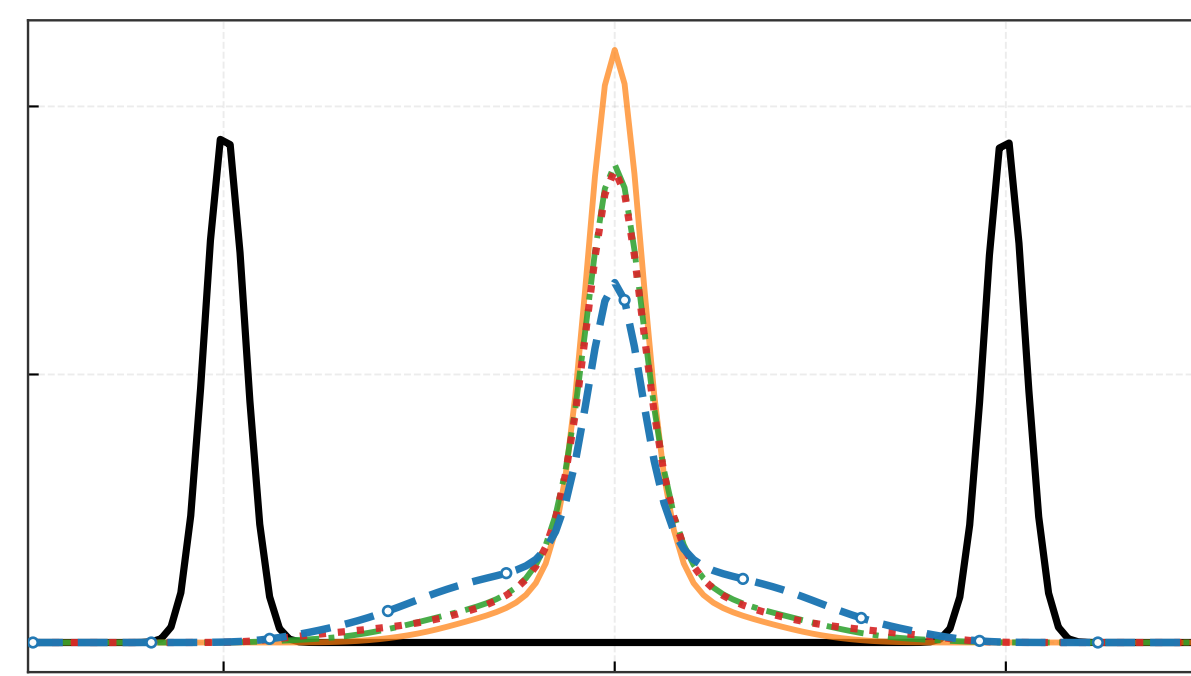
iteration 10
