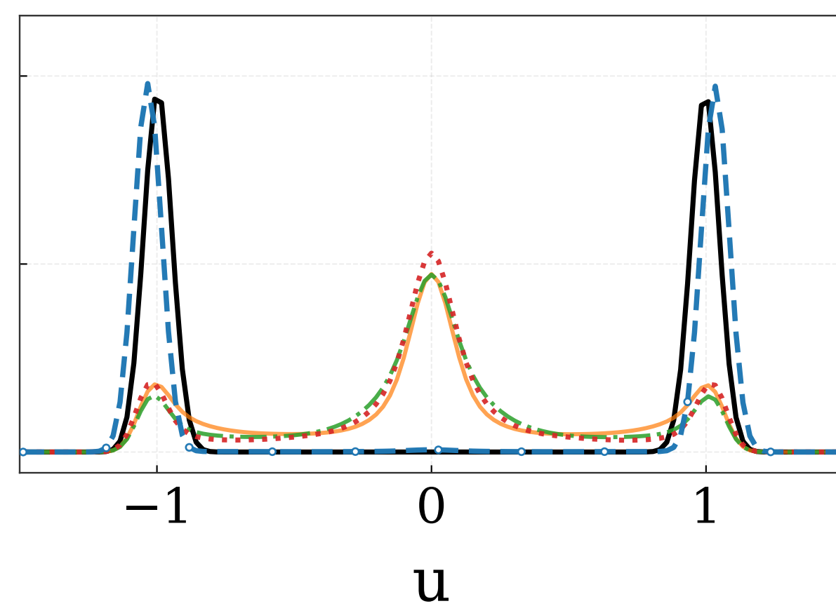
iteration 100
