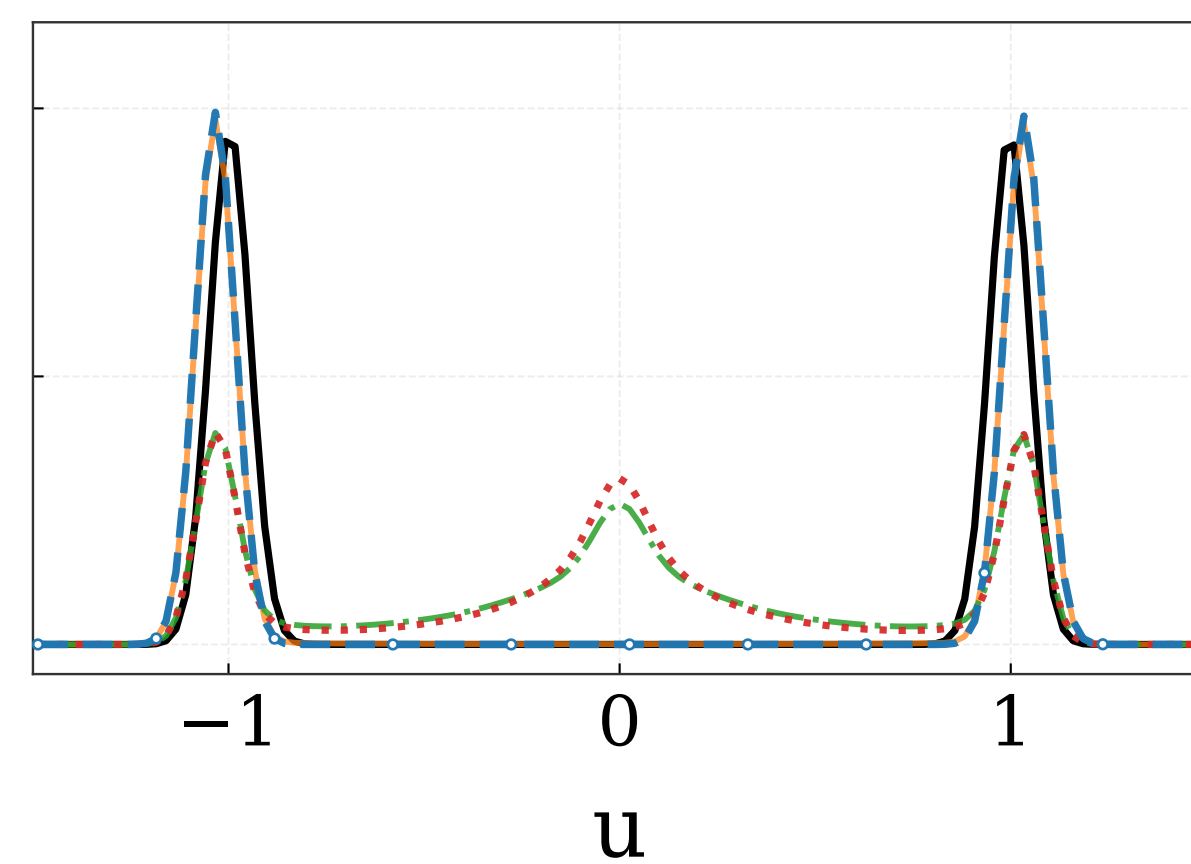
iteration 750
