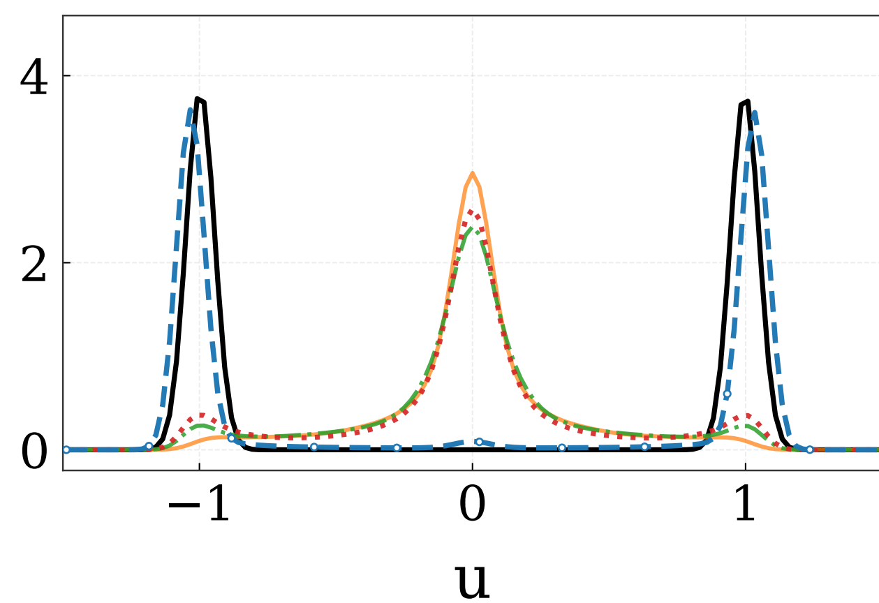
iteration 50
