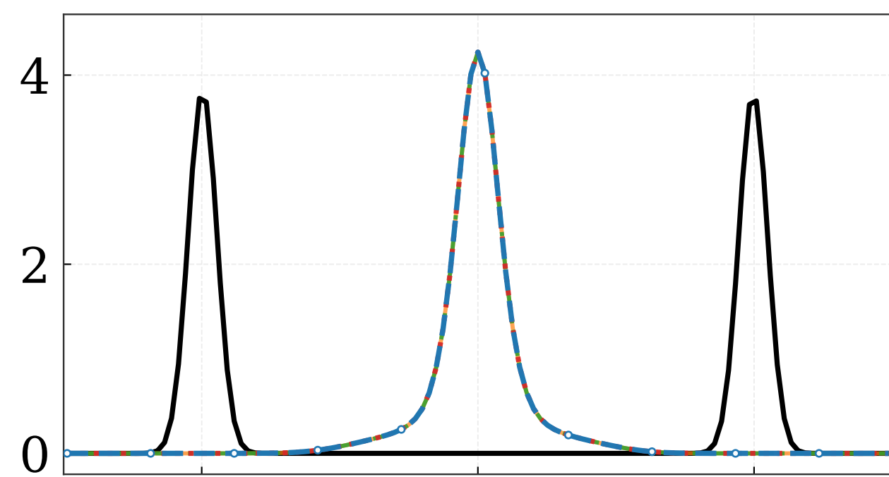
iteration 0
