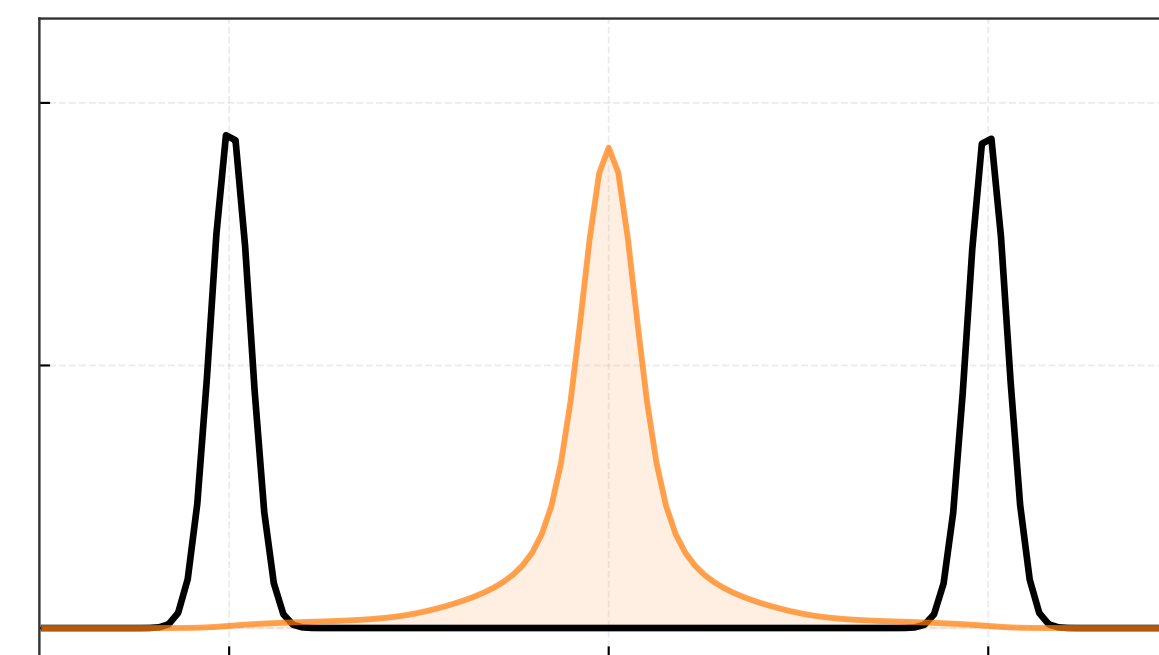
iteration 30
