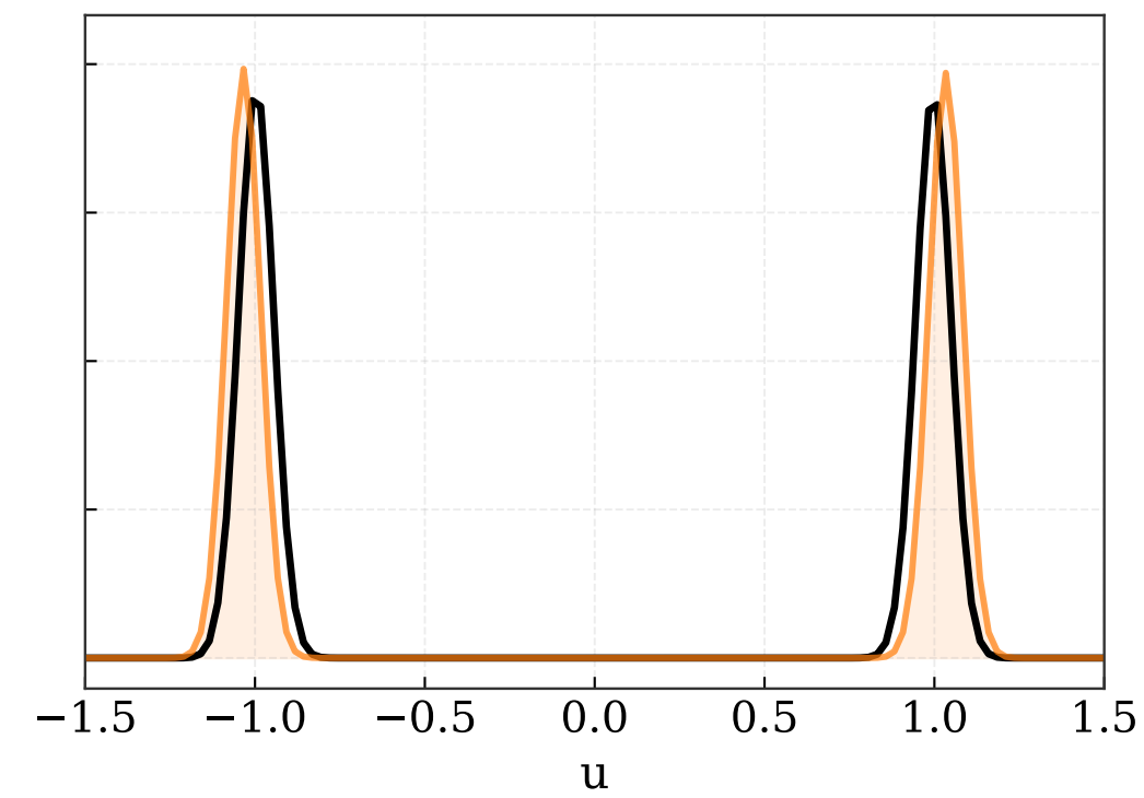
iteration 1500
