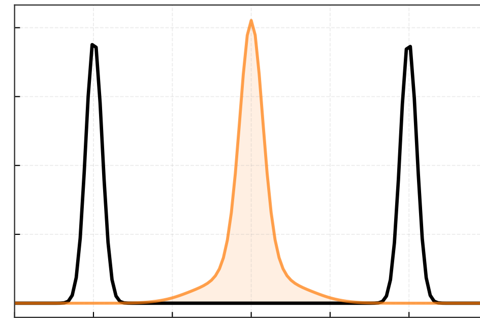
iteration 20
