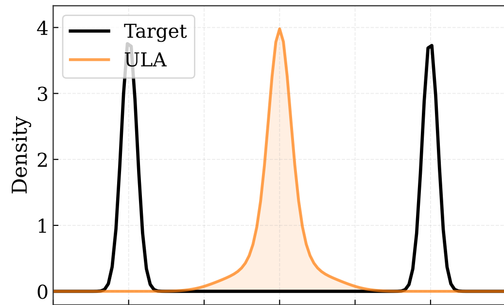
iteration 0
