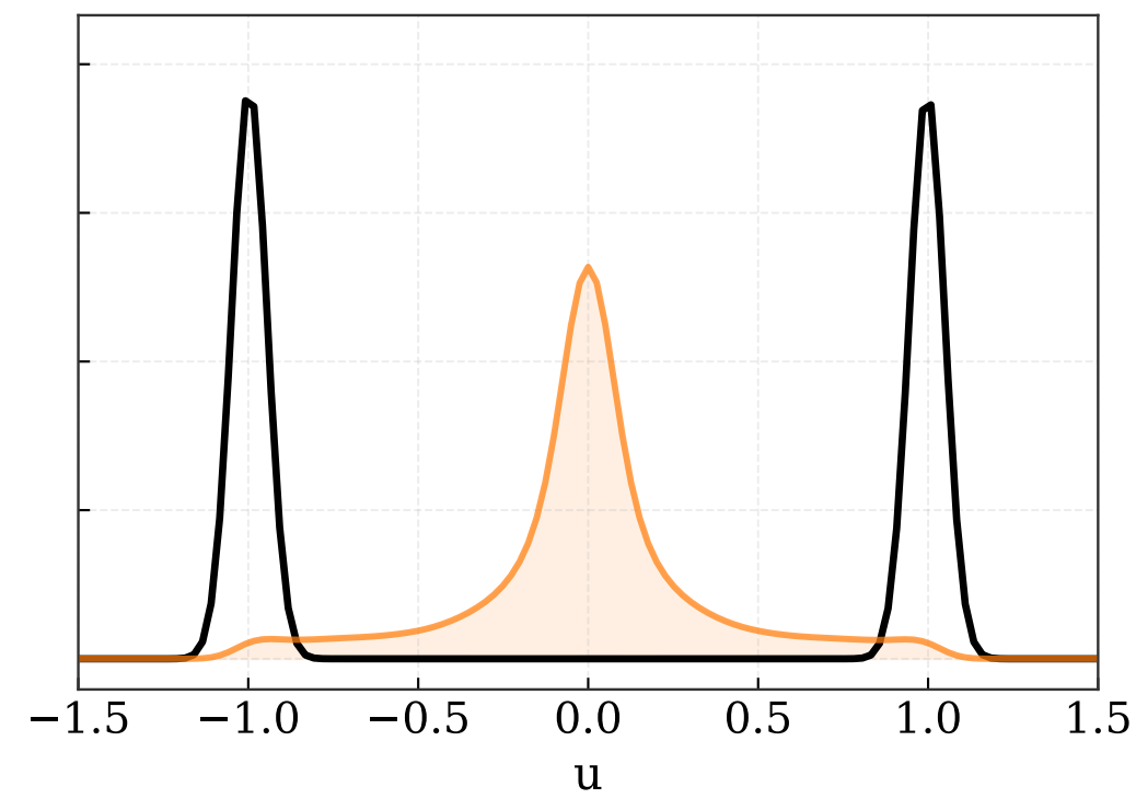
iteration 100
