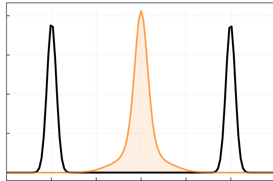
iteration 10
