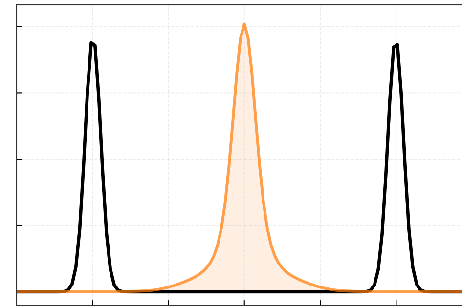
iteration 30
