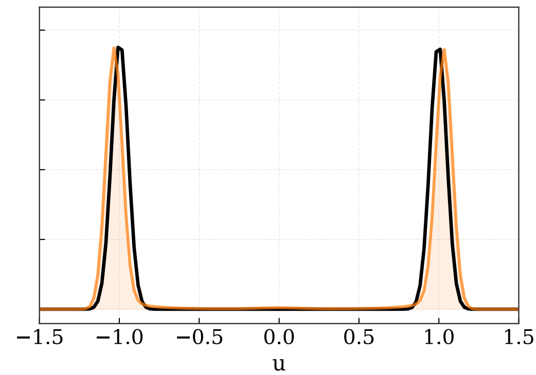
iteration 750
