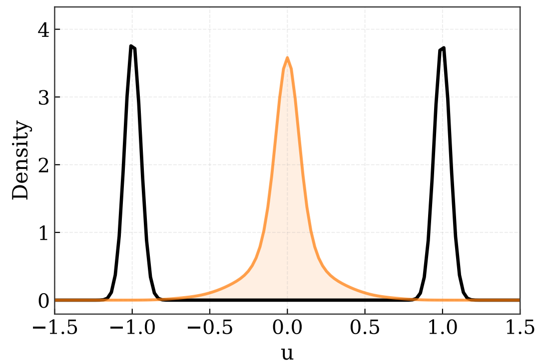
iteration 50
