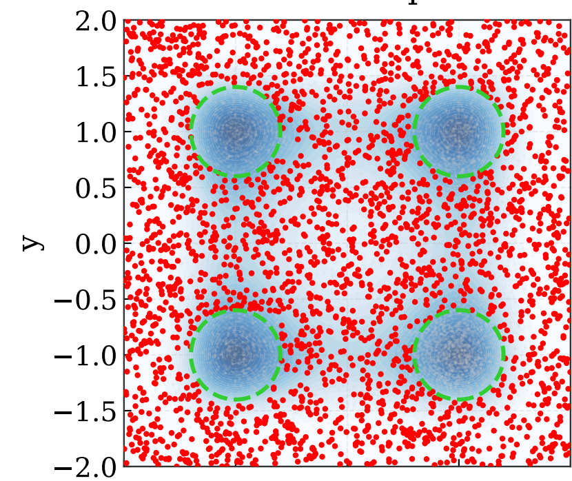
HMC: step 0
