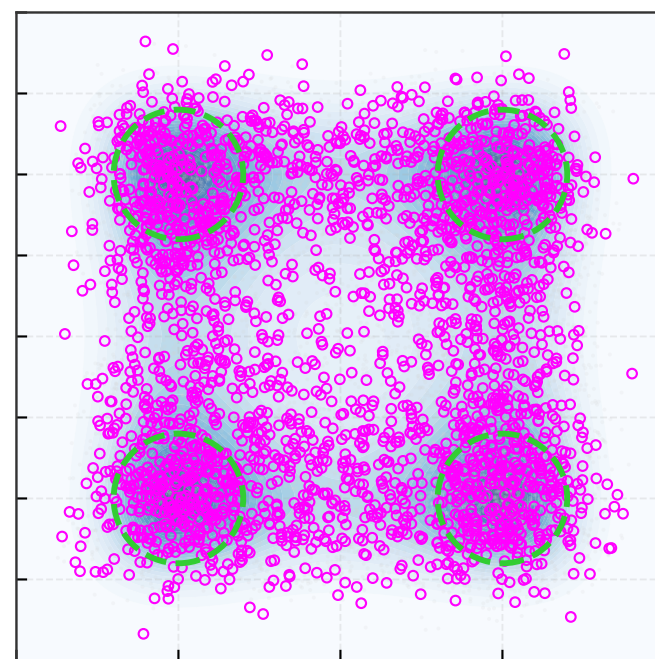
HMC: step 3000
