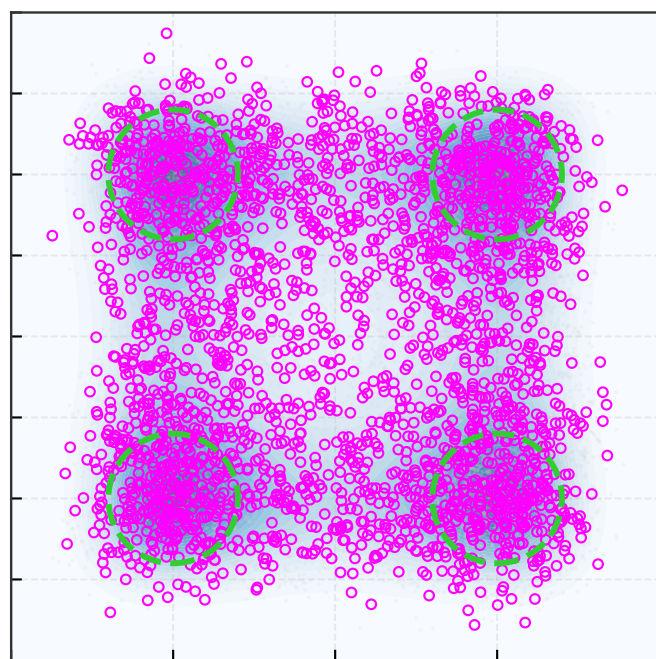
HMC: step 1000
