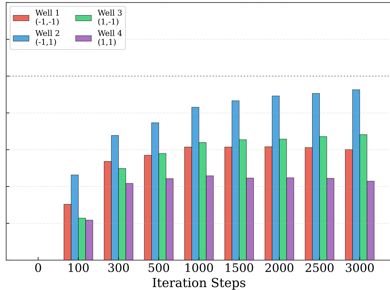
KSWGd: 4-Well Density Evolution
