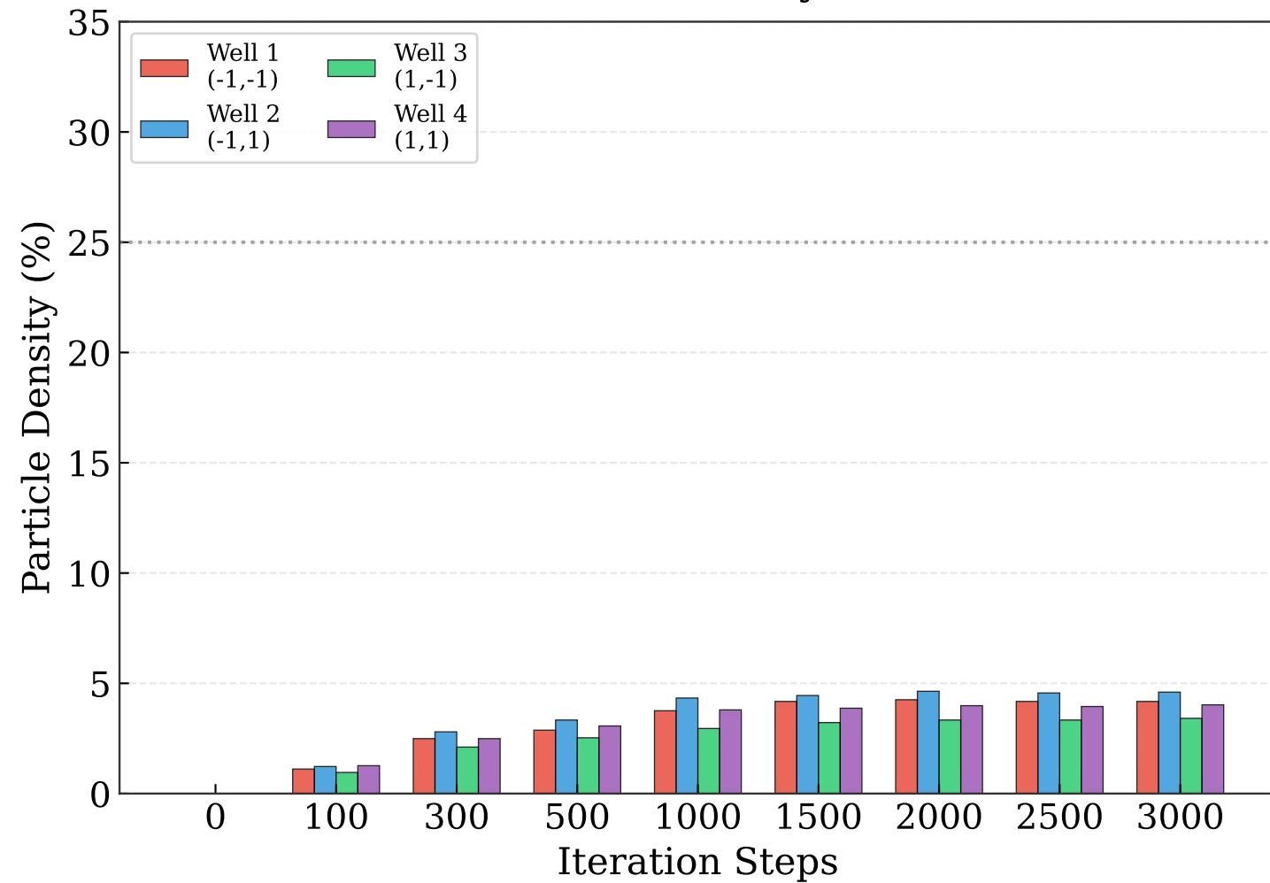
DMPS: 4-Well Density Evolution
