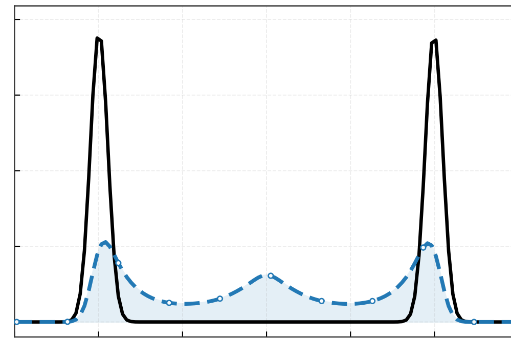
iteration 30
