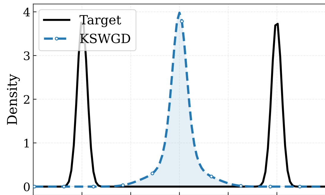
iteration 0
