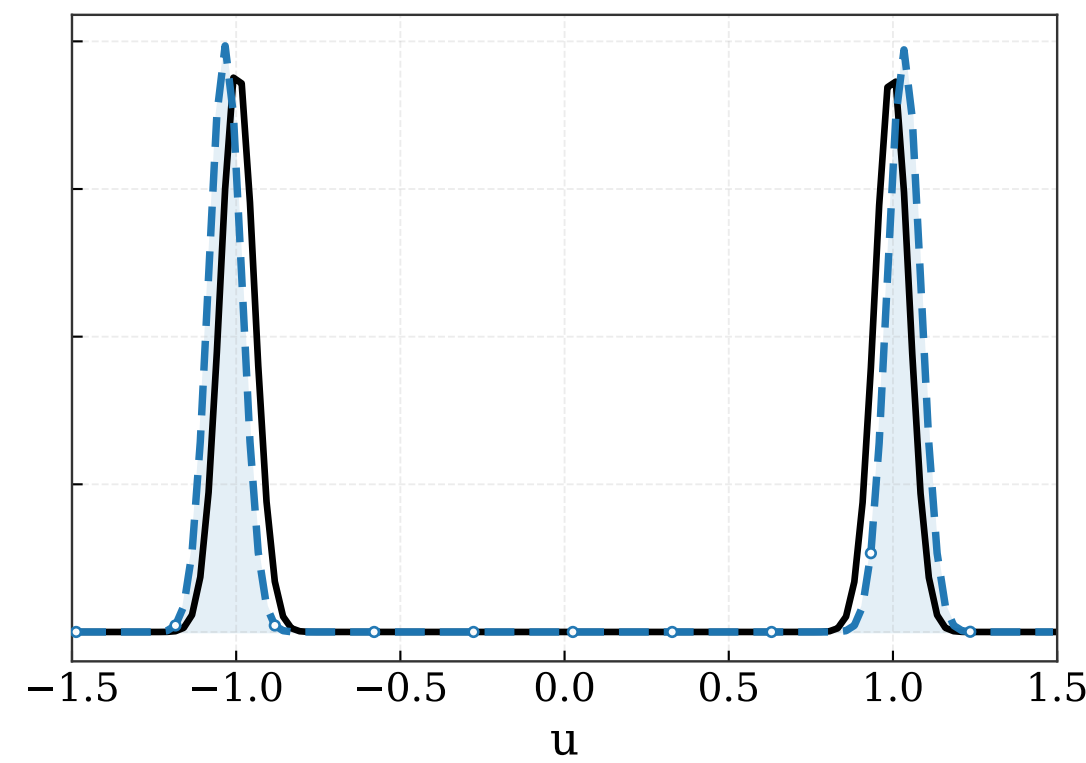
iteration 750
