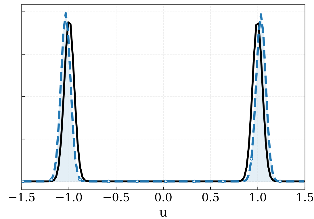
iteration 1500
