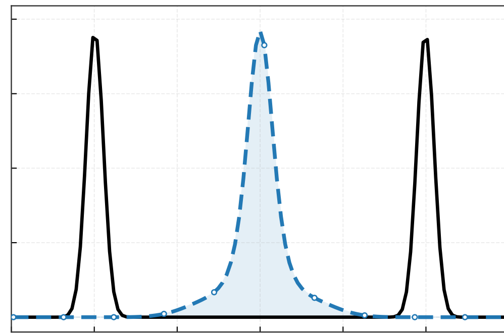
iteration 10
