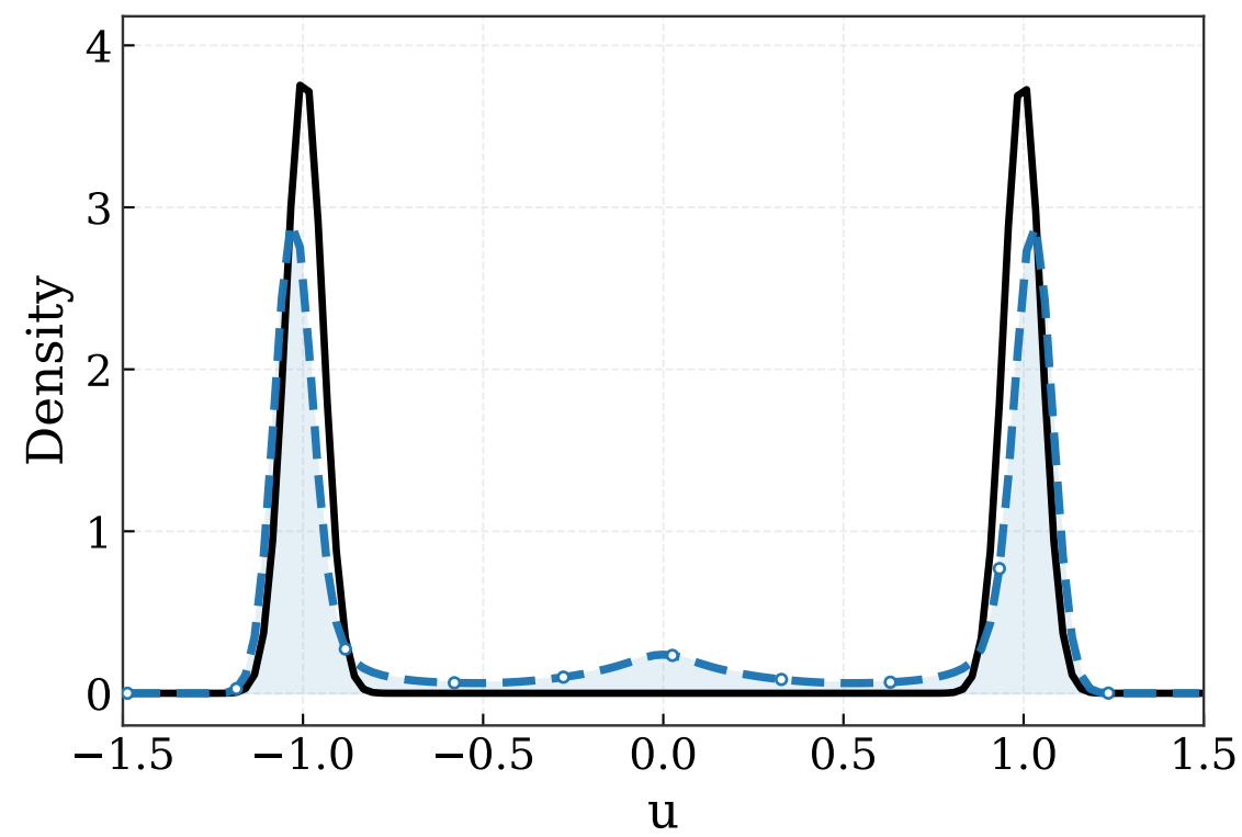
iteration 50
