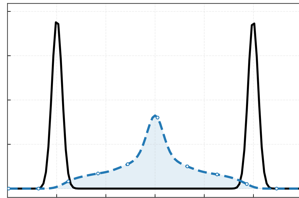
iteration 20
