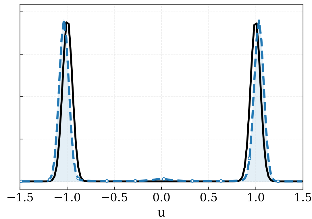
iteration 100
