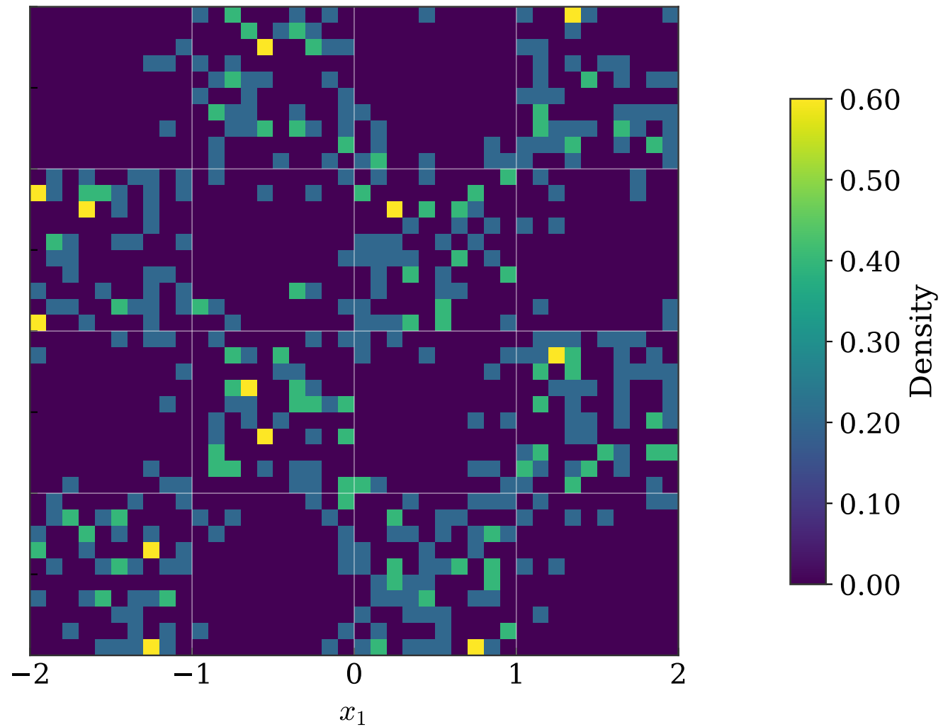
KSWGd final histogram
