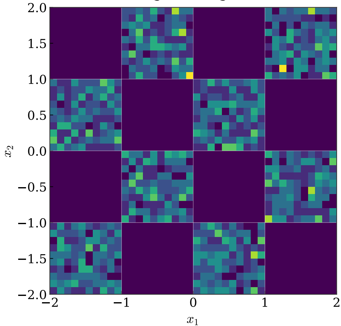
Target histogram
