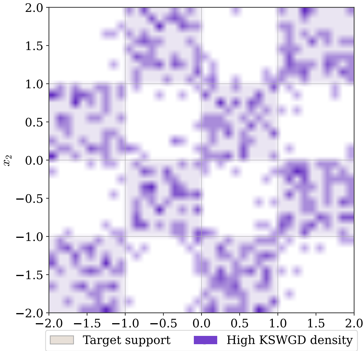
KSWG D Density on Chessboard
