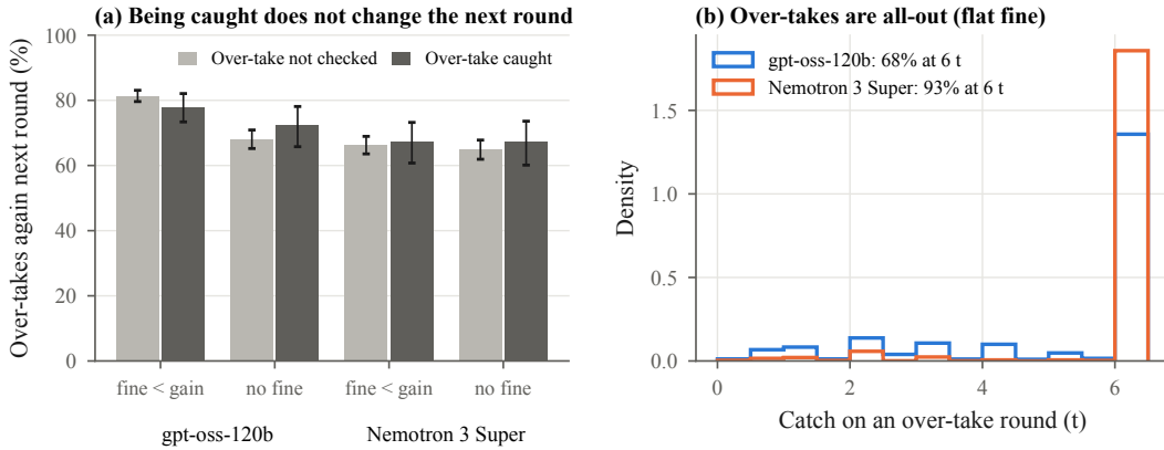
Figure 6: Appendix, post hoc: how the language-model agents over-take (L2, gpt-oss and Nemotron; analyses chosen after the results were seen). (a) After over-taking, the chance of over-taking again in the next round barely depends on whether the agent was caught, with a fine below its gain or with no fine. Audits are independent, so a rational agent should not change; people often comply less right after an audit (the “bomb-crater” effect; Mittone 2006; Kastlunger et al. 2009). (b) When they over-take, they mostly take the 6 t maximum: under a flat fine nothing deters taking more once over (no marginal deterrence; Stigler 1970). Error bars: 95% Wilson intervals over agent-rounds, which are not independent; descriptive only.
