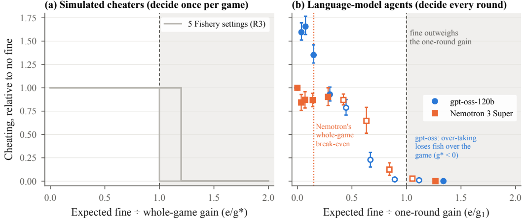
Figure 5: Each kind of agent stops cheating when the expected fine outweighs the gain it acts on. Shaded: the expected fine exceeds the gain on the horizontal axis. (a) Simulated cheaters choose one cheating level for the whole game, so they are scaled by their whole-game net gain g^* (gain over complying, per round of cheating). In five FISHERY settings they stop at e/g^* = 1.0 – 1.2 , as predicted before the search (R3). (b) Language-model agents decide every round, and are scaled by their one-round gain g_1 (extra tonnes in that round), measured with no fine. They stop close to e/g_1 = 1 : the stopping fine predicted from g_1 before L3 ran was exact for Nemotron and one grid step early for gpt-oss. They begin to cut back from about e/g_1 = 0.4 . Measured by the whole-game gain, they keep cheating far past the point where it pays. Over-taking loses gpt-oss fish over the game ( g^* < 0 ), and Nemotron’s whole-game break-even (dotted) lies at e/g_1 = 0.15 . They act on the gain of the round, not of the game. Filled: L2; open: L3. Error bars: 95% intervals over populations.
