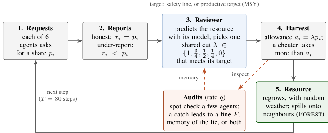
Figure 1: One step of the game. Six agents ask to take from a shared resource. The reviewer predicts what the requests would do and picks one cut for everyone that meets its target. Agents then harvest, and some may secretly take more than allowed. Audits spot-check a few agents and turn what they find into consequences: a fine, a memory of the lie, or both. Table 1 defines every term.
