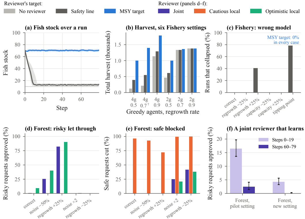
Figure 2: What the reviewer aims for, and what it knows, decide how well it protects the resource. Top row, FISHERY: (a) fish stock over one run when the reviewer sees all requests (4 greedy agents; line: middle run, band: 80% of 64 populations). With only the safety line, the stock is fished down to just above 10; with the MSY target it stays near 70. (b) Total harvest in six settings (“4g 0.7” = 4 greedy agents, regrowth 0.7; † the pilot setting). The MSY target gives more wherever the safety line limits anything (1,394 against 544 in the pilot setting). (c) Share of runs in which the stock collapsed when the reviewer’s model is wrong: 41% (regrowth overestimated) and 78% (an unknown tipping point) with the safety line, 0% with the MSY target. Bottom row, FOREST: (d) risky requests let through and (e) safe requests blocked, when one part of the reviewer’s model is wrong. The direction of the error decides the mistake: thinking regrowth is faster lets 82% of risky requests through; thinking it slower blocks 42% of safe ones. The cautious local reviewer blocks most safe requests in every case. (f) A joint reviewer that learns the model while running lets through 16% of risky requests early and 2.5% late. Error bars: 95% intervals.
