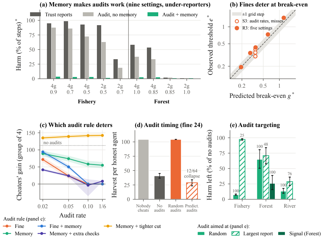
Figure 3: What makes audits work: memory, an expected fine above the gain, and audits that reach everyone. (a) Under-reporters in nine settings (one random audit per step, no fines). Auditing without memory barely reduces harm; remembering each caught lie removes most of it. *FISHERY: steps above the MSY limit; FOREST: steps below the safety line. (b) FISHERY: the expected fine at which cheaters stop ( e^* ) against the break-even predicted from no-check runs ( g^* , the gain from one step of cheating). Filled: five settings, predicted before the search (R3). Open: the pilot setting at audit rates from 1/6 to 0.02 and with audits that miss three cheats in four (S3). Every point lies within one grid step (shaded) of the prediction. (c) Cheaters' gain as the audit rate rises, under five audit rules (fine 6; bands: 95% intervals). A fine stops cheating from an audit rate of 0.10; memory alone leaves about half the gain; tightening everyone's cut to allow for known cheaters makes cheating pay more than with no audits. (d) Harvest per honest agent at the same audit rate (1/6) and fine (24): random audits stop cheating; predictable audits (every agent on every sixth step) leave honest agents worse off than no audits (28.8 against 40.9). (e) Harm left, as a share of the harm with no audits, when one audit per step (with memory) is aimed at random, at the largest report, or, in FOREST, at the plot doing worst against prediction. Numbers above the bars: the share of liars ever caught. Aiming at the largest report keeps auditing the same agent, so in FISHERY only 25% of liars are ever caught and harm stays at 97% of the no-audit level. Error bars: 95% intervals.
