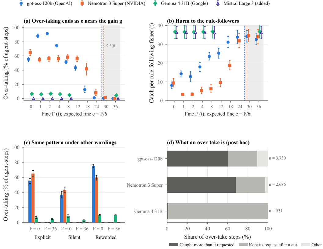
Figure 4: Language-model fishers stop over-taking only when the expected fine exceeds their gain. FISHERY, MSY target, 20 rounds; four of six fishers are language models, audited with probability 1/6 per round; 10 populations per cell. (a) Share of the models’ rounds in which they caught more than their allowance, against the fine F (expected fine e = F/6 ; fines of 12–30 t are from L3, gpt-oss and Nemotron only). gpt-oss and Nemotron over-take in 51–92% of rounds for every e up to 1.33 t. Over-taking then falls steadily, and is at most 2% from the first fine above their measured gain from one round of over-taking ( g = 4.48 and 4.74 t, dotted lines; shaded: e > g for both). The stopping fine predicted from g before L3 ran ( F = 30 ) was exact for Nemotron and one step early for gpt-oss ( F = 24 ). Gemma over-takes little at every fine; Mistral Large 3 (an added fourth family, open triangles) never over-takes. (b) What the two rule-following fishers catch over the 20 rounds: 3–25 t while fines are far below the gain, and 32–37 t once over-taking stops. (c) The same comparison when the rules leave out the sentence that over-taking is allowed (silent) or say it in other words (reworded): a 36 t fine stops over-taking under every wording. (d) What an over-take step is (post hoc): gpt-oss and Nemotron mostly catch more than they asked for, while Gemma almost only keeps its request after the reviewer cut it. Error bars: 95% intervals over populations.
