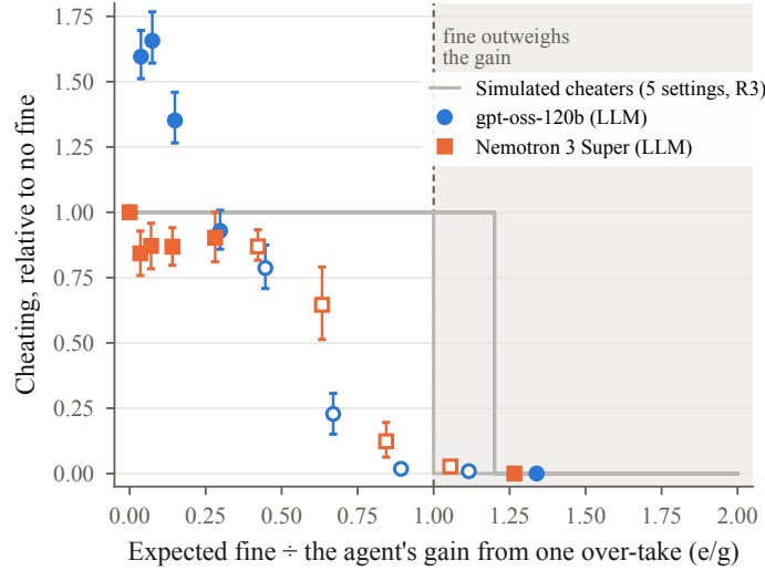
Figure 5: Programmed and language-model agents stop cheating at the same point: when the expected fine outweighs their own gain. The horizontal axis is the expected fine divided by the agent’s gain from one step of over-taking, e/g , measured with no fine; to the right of the dashed line, cheating does not pay. Grey: the cheating level chosen by simulated cheaters in five FISHERY settings (R3), relative to their level with no audits; the threshold was predicted before the search. Markers: how often gpt-oss and Nemotron over-take at each fine, relative to no fine (filled: L2; open: L3, whose fines fall between e/g = 0.4 and 1.1 and whose stopping point was predicted in advance). The language models stop close to e/g = 1 , but unlike the simulated best-responders they start to cut back from about e/g = 0.4 : they are easier to deter than a risk-neutral agent. Error bars: 95% intervals over populations.
