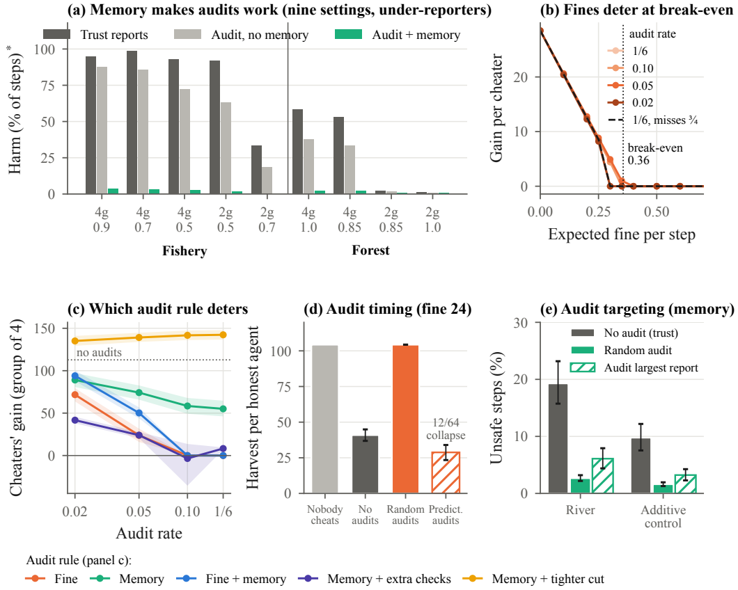
Figure 3: What makes audits work: memory, an expected fine above the gain, and unpredictable targets.
