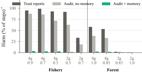
(a) Memory makes audits work (nine settings, under-reporters)
