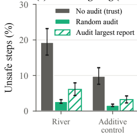
(e) Audit targeting (memory)
