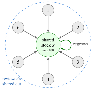
(a) FISHERY: a star
