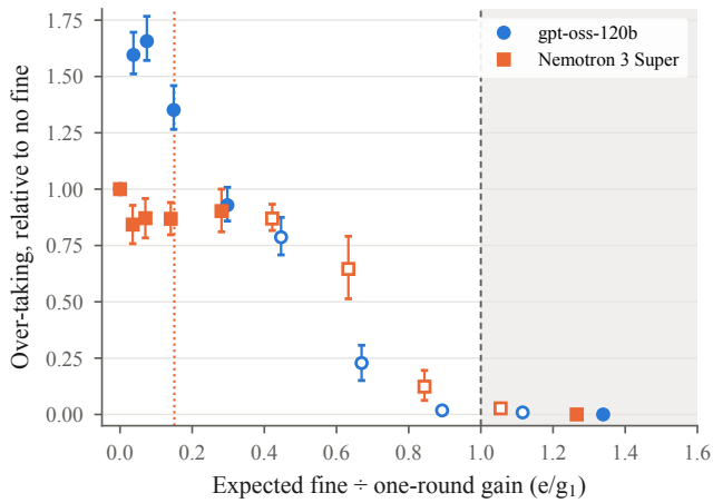
Figure 4: Over-taking by gpt-oss-120b and Nemotron 3 Super, relative to no fine, against the expected fine divided by each model’s one-round gain g_1 . Open markers show the fines of the threshold test, whose stopping point was predicted in advance; the shaded area marks fines above g_1 . The dotted line marks Nemotron 3 Super’s whole-game break-even; gpt-oss-120b’s whole-game gain was negative. Programmed cheaters, which commit to one level per game, stopped at 1.0–1.2 of their whole-game gain (Figure 2b).
