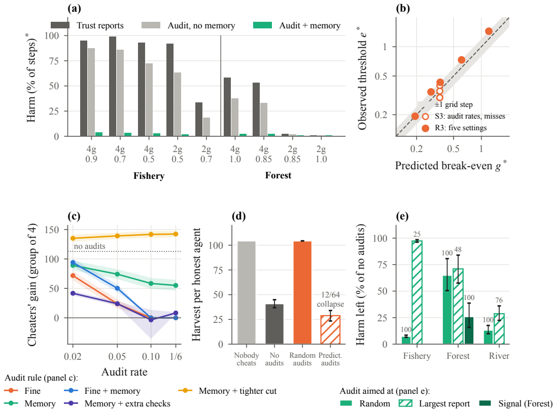
Figure 2: Audits with programmed agents. (a) Share of rounds below the harm line with under-reporters in nine settings (Fishery and Forest; 2 or 4 greedy agents and regrowth rate), when the reviewer trusts reports, audits without memory, or audits with memory. (b) Observed deterrence threshold e^* against the break-even g^* predicted from runs without audits; filled points are five settings predicted before the search, open points are audit rates from 1/6 to 0.02 and audits that miss cheats; the band marks one grid step. (c) Cheaters' gain against audit rate under five audit rules; the dotted line marks no audits. (d) Harvest per honest agent with a fine of 24 under random and predictable audits. (e) Harm remaining, relative to no audits, when one audit per round is aimed at random, at the largest report, or at the plot doing worst against prediction; numbers give the share of liars ever caught. Error bars and bands show 95% intervals over populations.
