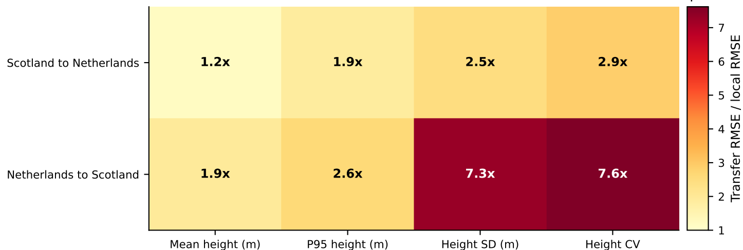
e Transfer error relative to a model trained and tested within the destination landscape
