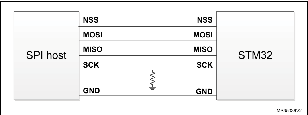
Figure 4. SPI connection
