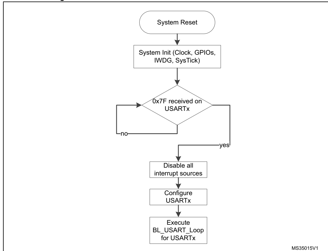
Figure 18. Bootloader selection for STM32F03xx4/6 devices
