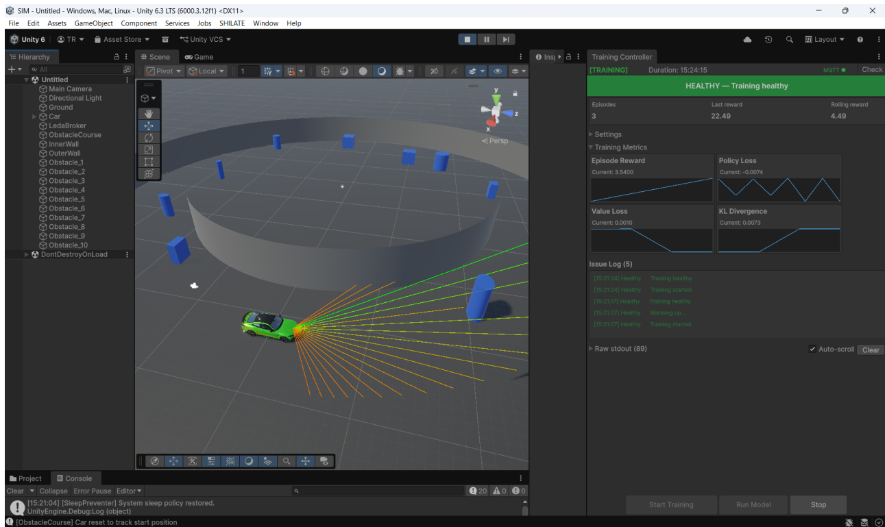
Figure 4.3: Unity Editor during a live training session. The Scene view shows the obstacle course with the 21-ray LiDAR fan, the circular track walls, and the vehicle. The Training Controller panel displays the HEALTHY banner, episode metrics, and live loss graphs.
