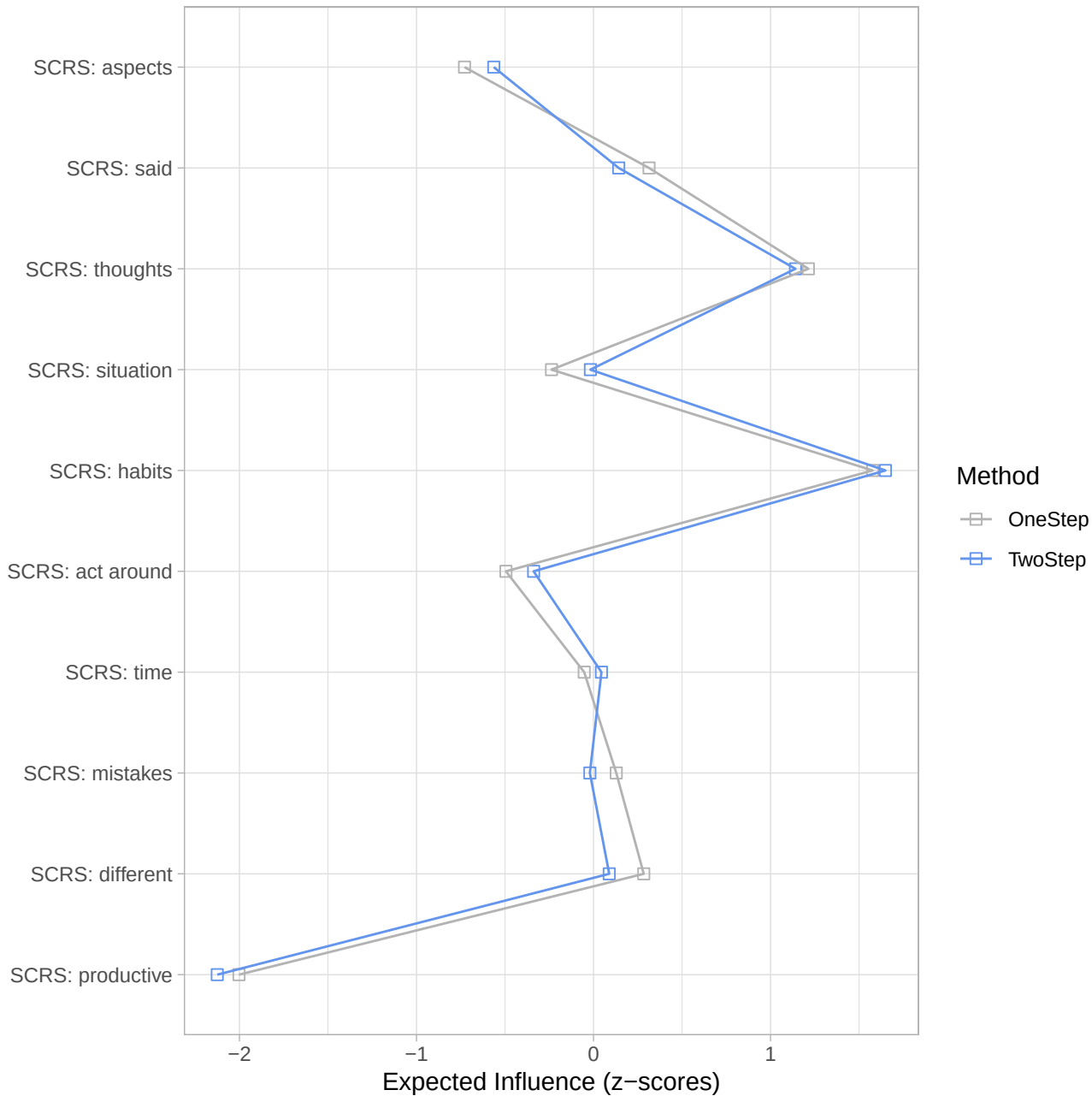
One- and Two-Step Expected Influence estimates for SCRS
