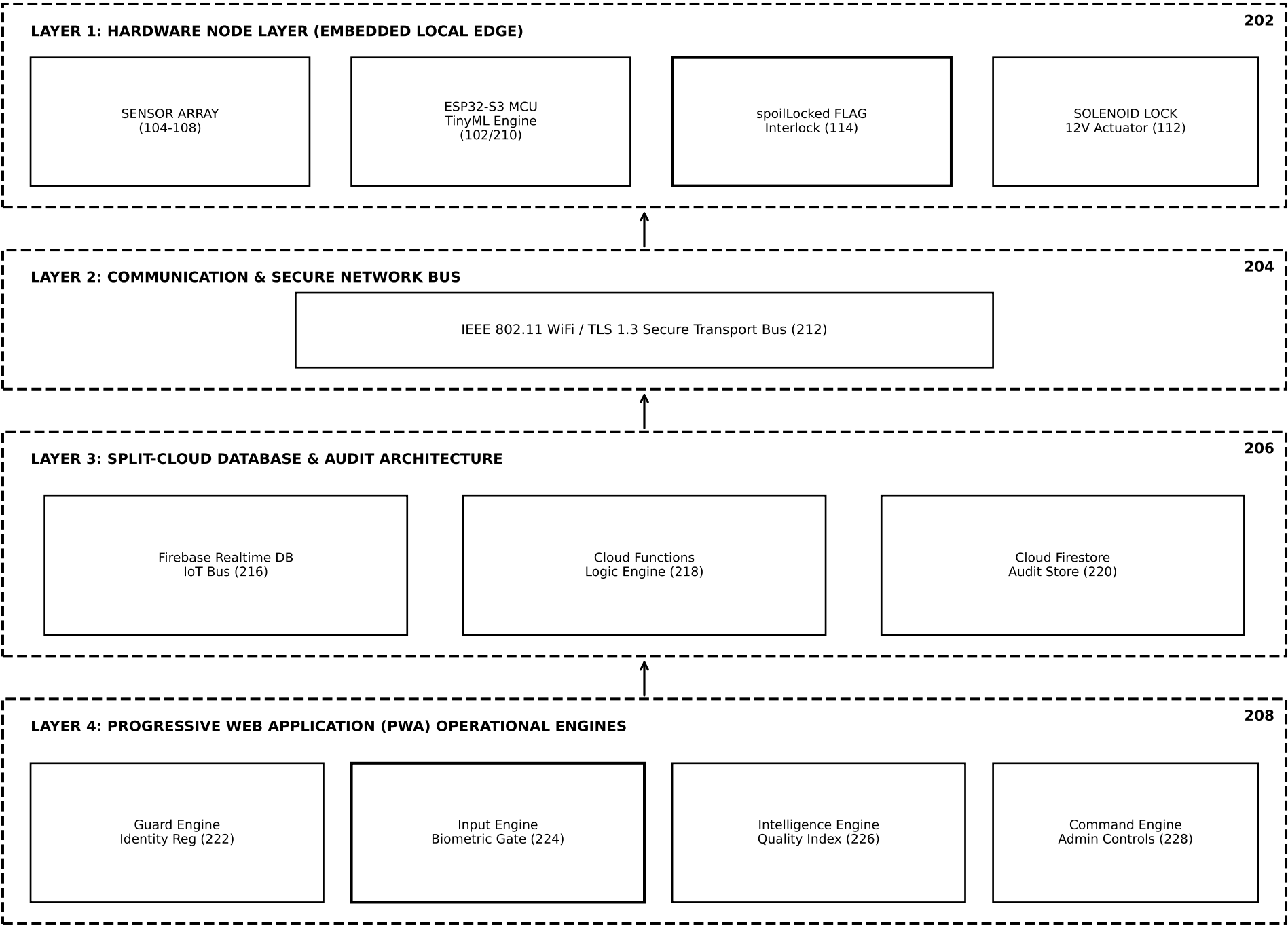
FOUR-LAYER SYSTEM ARCHITECTURE
